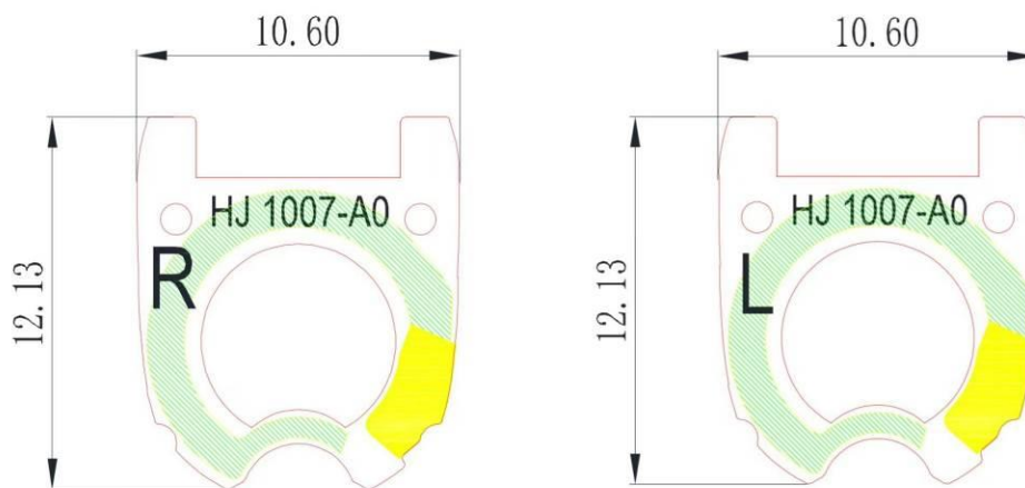
Antenna Dimensions
