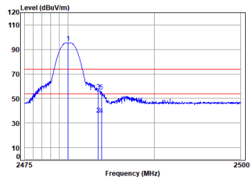
Right BLE_1M_TX_CH_39_Vertical
