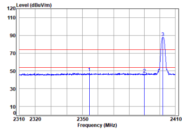
Left BLE_1M_TX_CH_00_Vertical
