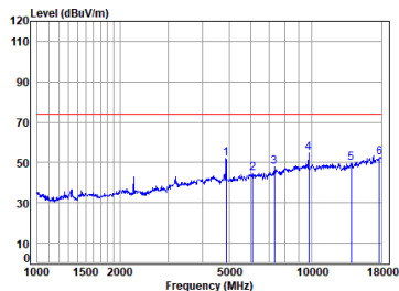
01 BLE_1M_TX_CH_19_Vertical-Peak
