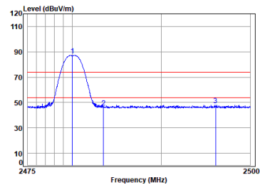
Left BLE_1M_TX_CH_39_Vertical
