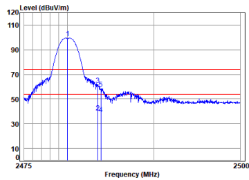
Right BLE_1M_TX_CH_39_Horizontal
