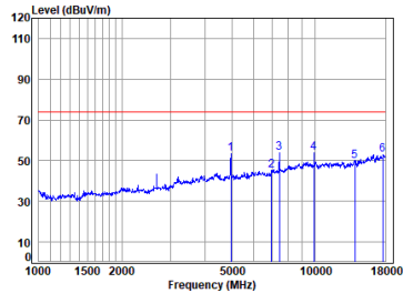
01 BLE_1M_TX_CH_39_Horizontal-Peak
