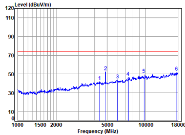
01 BLE_1M_TX_CH_19_Horizontal-Peak
