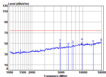
01 BLE_1M_TX_CH_19_Horizontal-Peak
