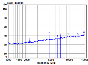
01 BLE_1M_TX_CH_00_Horizontal-Peak
