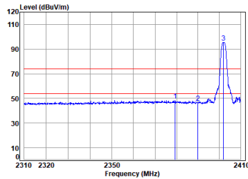
Left BLE_1M_TX_CH_00_Horizontal
