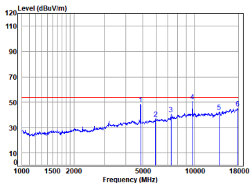
01 BLE_1M_TX_CH_19_Vertical-Avg
