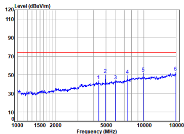
01 BLE_1M_TX_CH_39_Vertical-Peak
