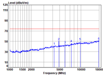
01 BLE_1M_TX_CH_19_Vertical-Peak
