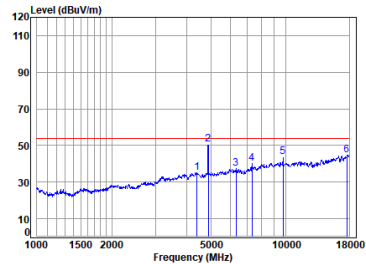
01 BLE_1M_TX_CH_19_Vertical-Avg
