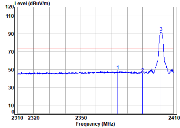
Right BLE_1M_TX_CH_00_Vertical
