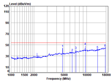
01 BLE_1M_TX_CH_00_Vertical-Avg
