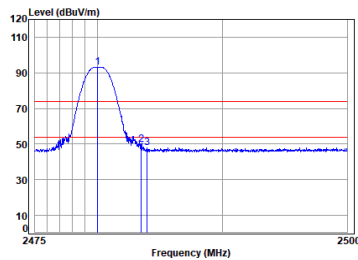
Left BLE_1M_TX_CH_39_Horizontal
