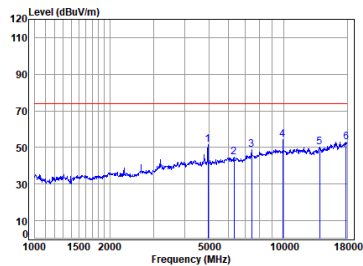
01 BLE_1M_TX_CH_39_Vertical-Peak
