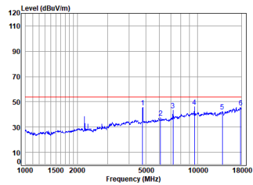
01 BLE_1M_TX_CH_00_Horizontal-Avg
