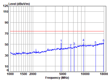
01 BLE_1M_TX_CH_00_Vertical-Peak
