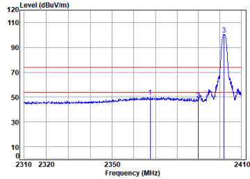
Right BLE_1M_TX_CH_00_Horizontal
