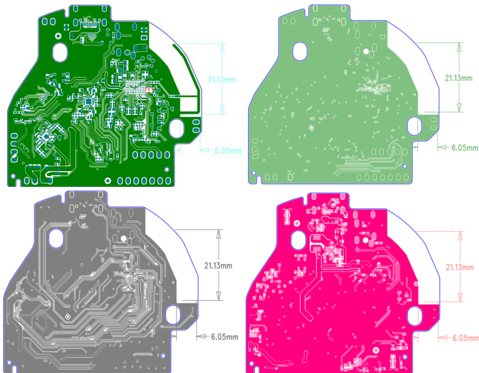
Antenna Dimensions
