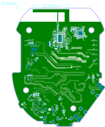
Antenna Dimensions
