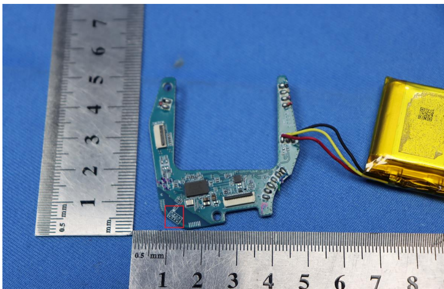
Antenna location:
