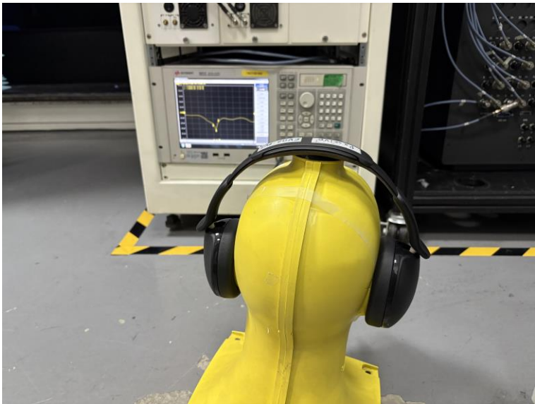
Free Space Impedance Setup
