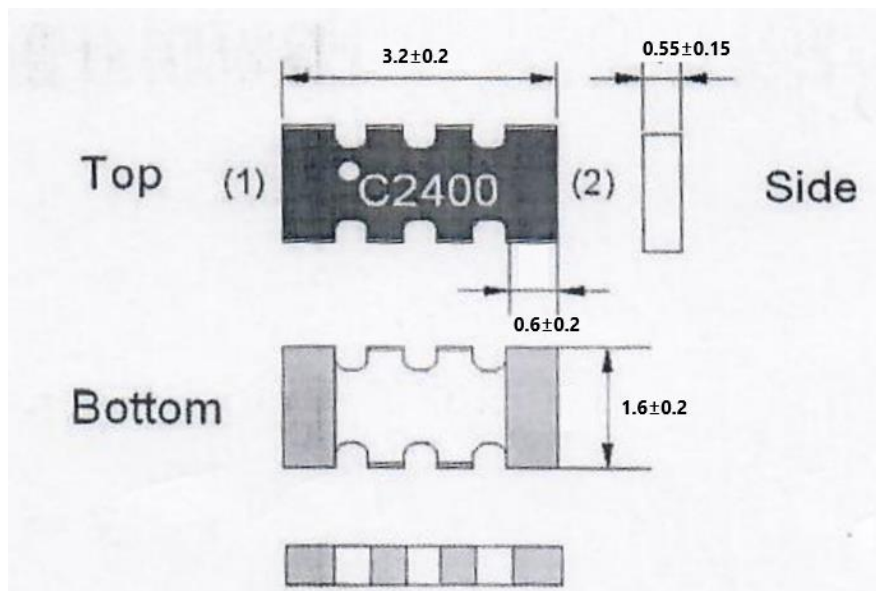
Antenna Dimensions
