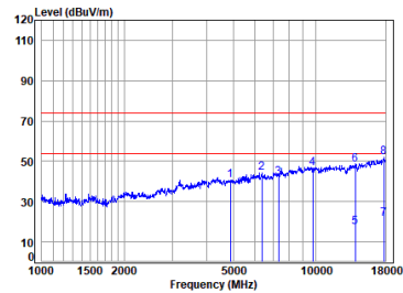
BT_DH5_TX_CH_39_Vertical
