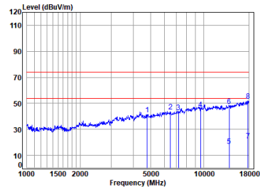
BT_DH5_TX_CH_00_Vertical
