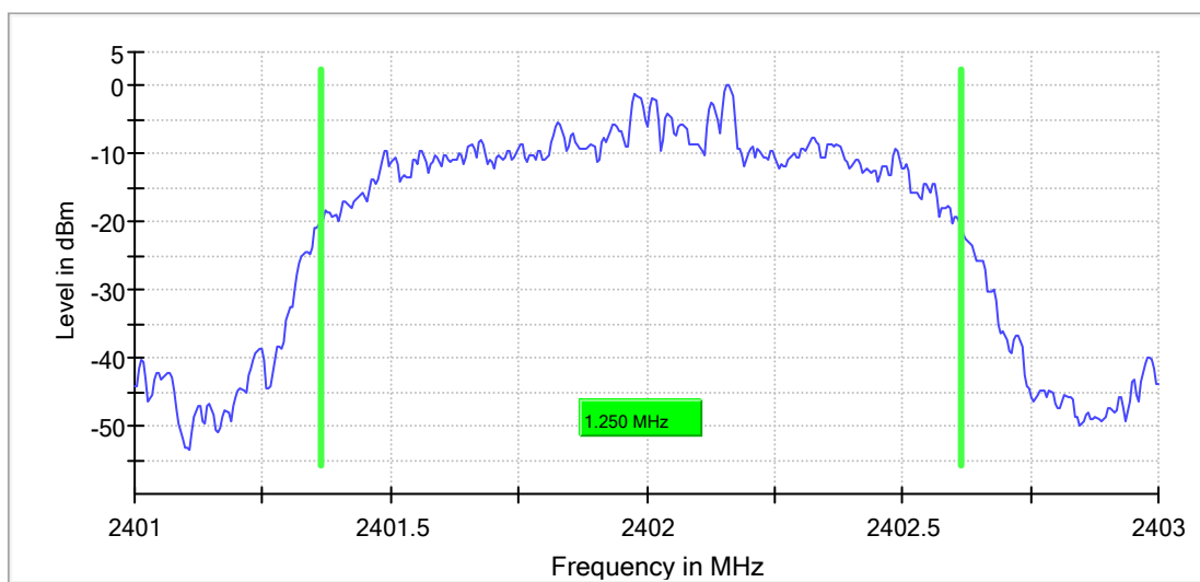
3DH5_Ant1_2402
