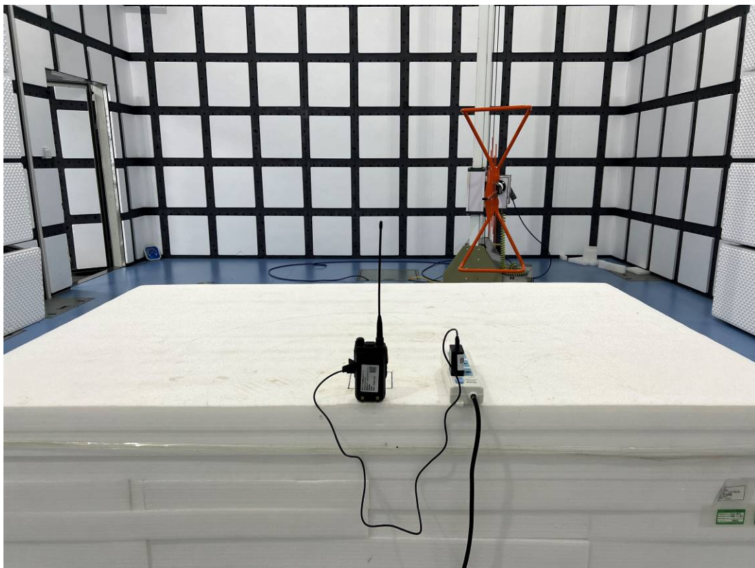
RE - Back View (Below 1GHz) - Mode 2
