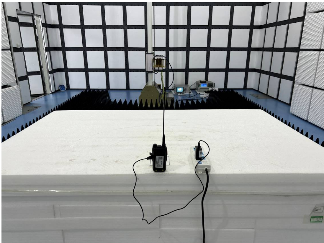
RE - Back View (Above 1GHz) - Mode 2
