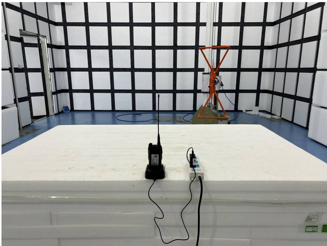
RE - Back View (Below 1GHz) - Mode 1
