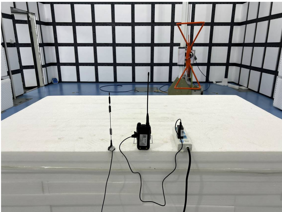
RE - Back View (Below 1GHz) - Mode 4
