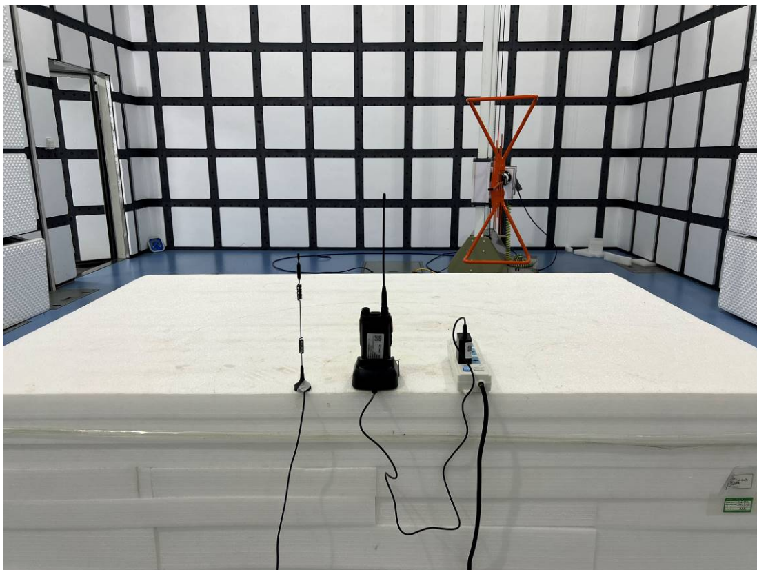
RE - Back View (Below 1GHz) - Mode 3
