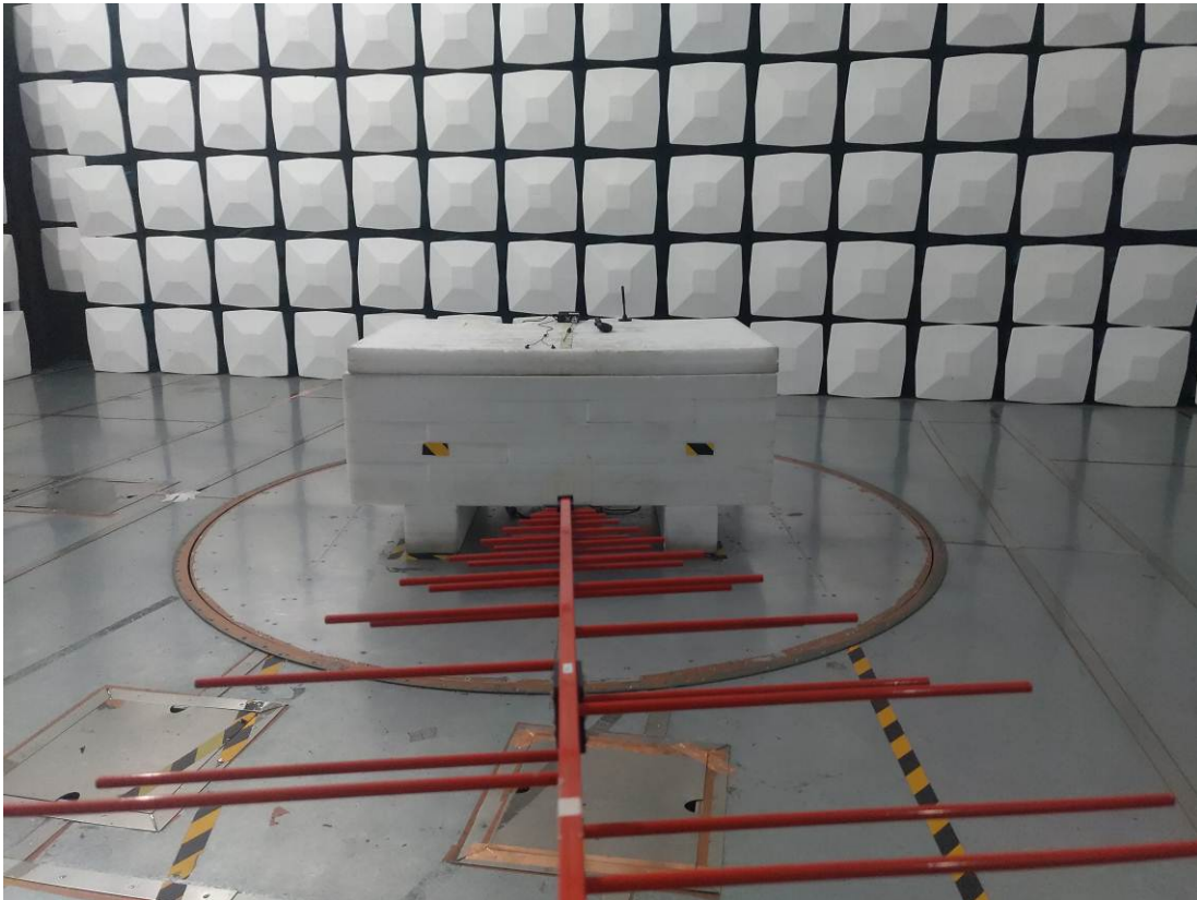
Radiated Emission 30M-1GHz Rear View-Mode 2
