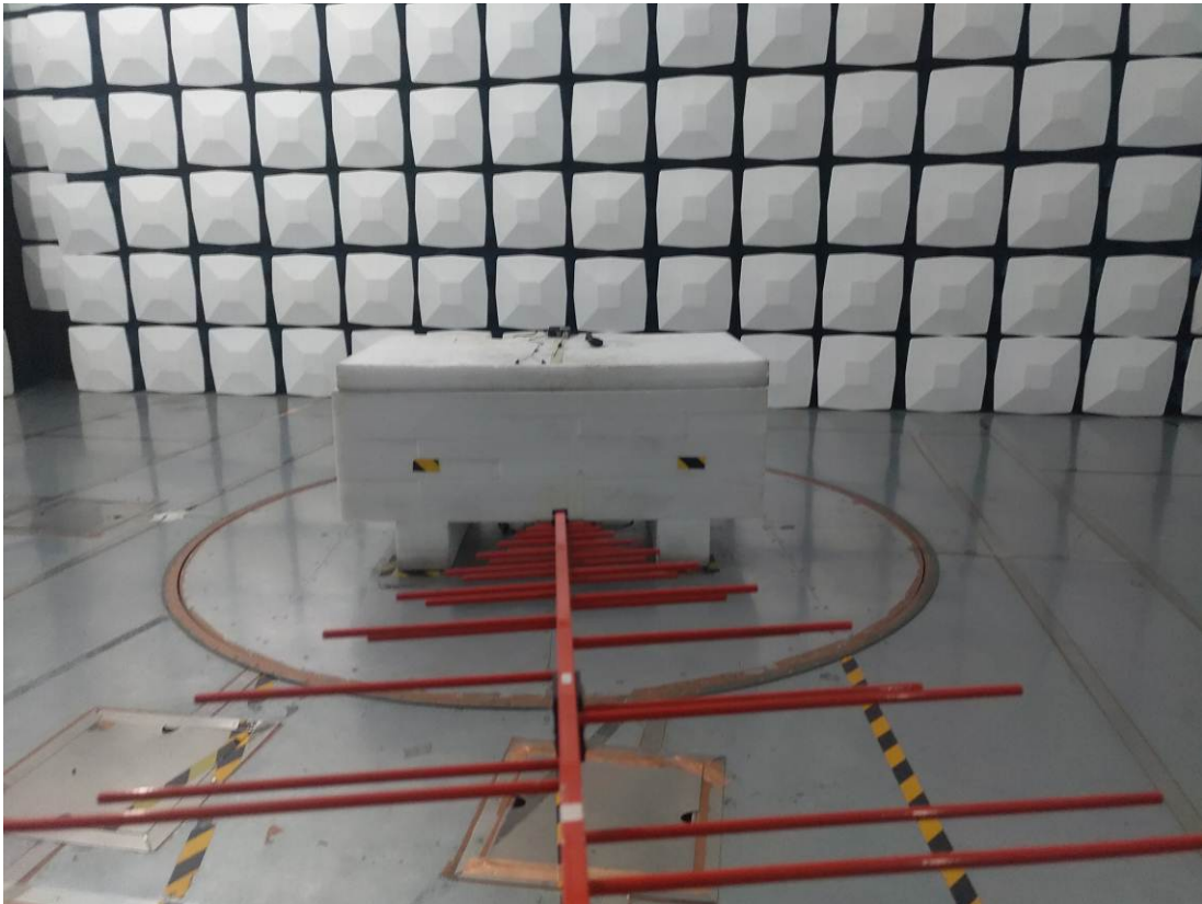
Radiated Emission 30M-1GHz Rear View-Mode 1
