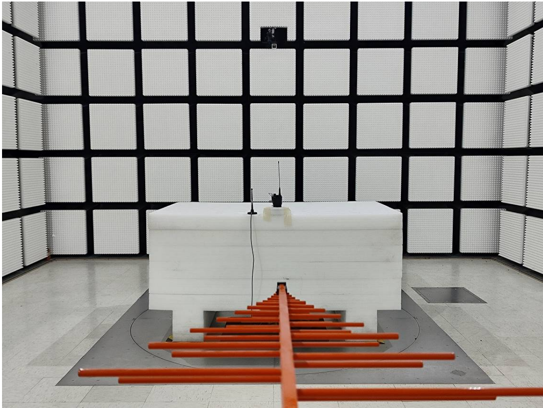
Radiated Emission Below 1GHz rear View M2-M7
