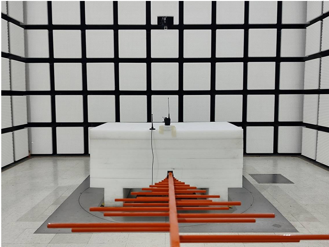
Radiated Emission Below 1GHz rear View M3-M6
