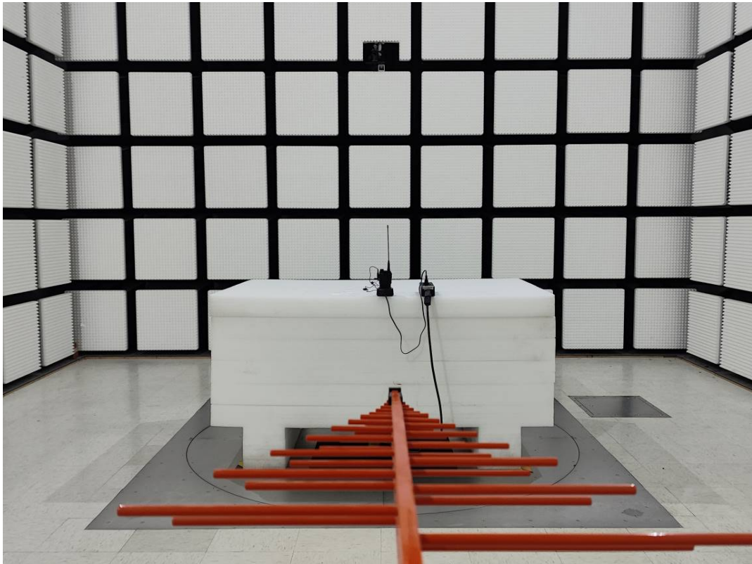
Radiated Emission Below 1GHz rear View M2
