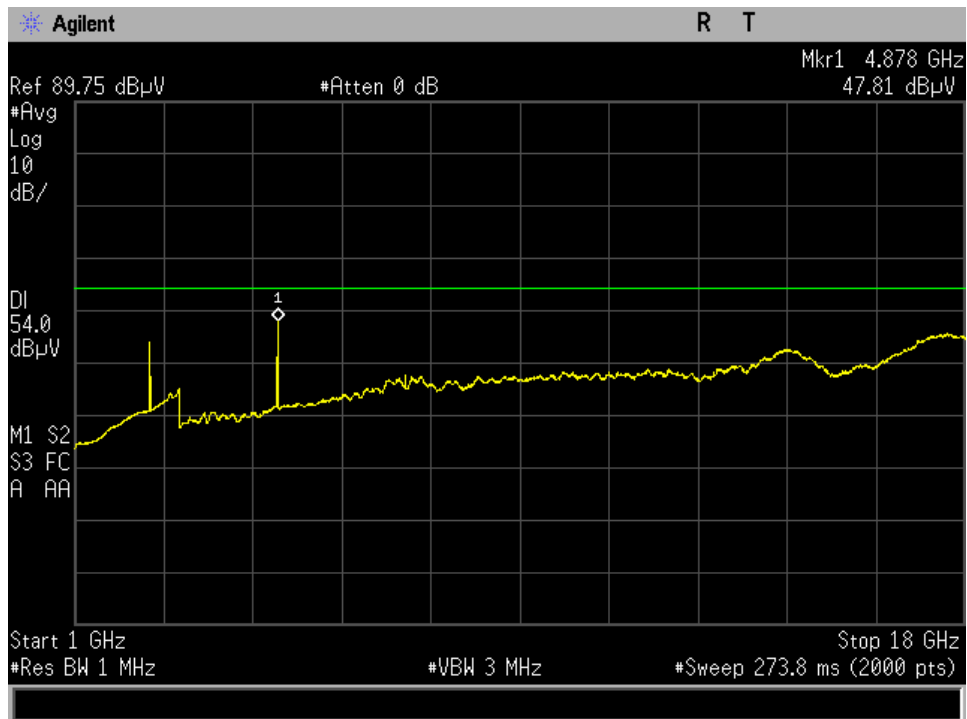
1-18 GHz Middle Channel outside antenna Peak
