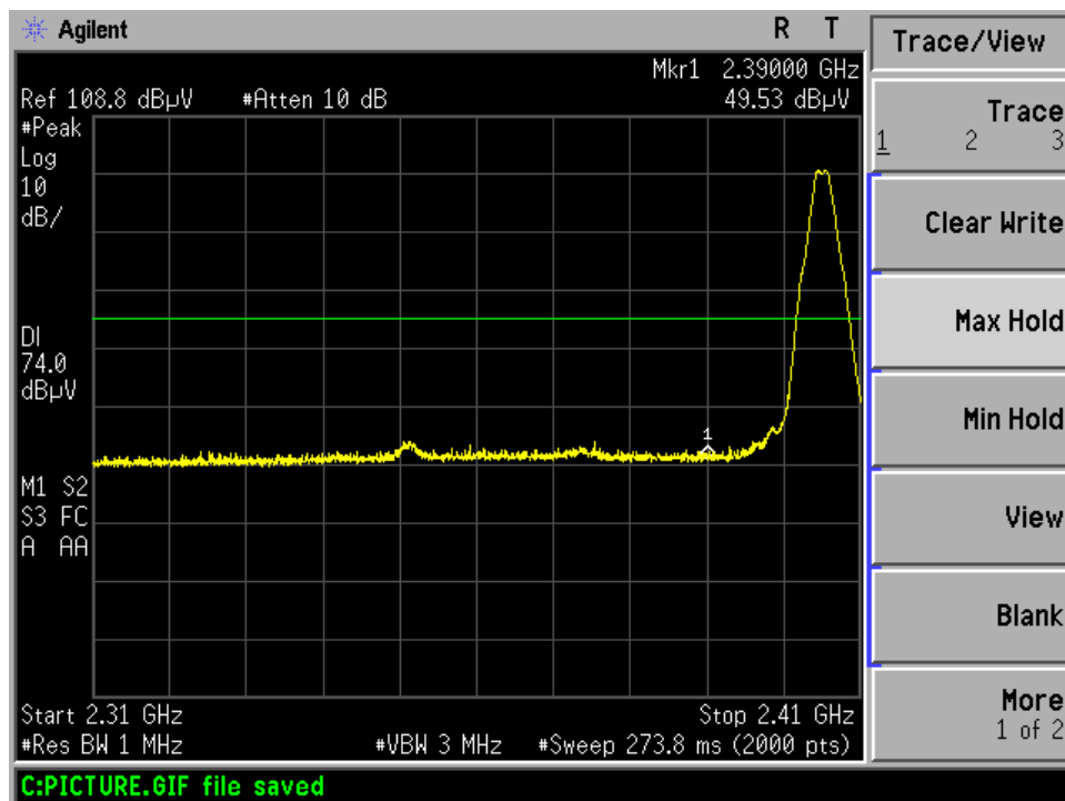
low Channel restricted Band edge Inside Antenna Peak
