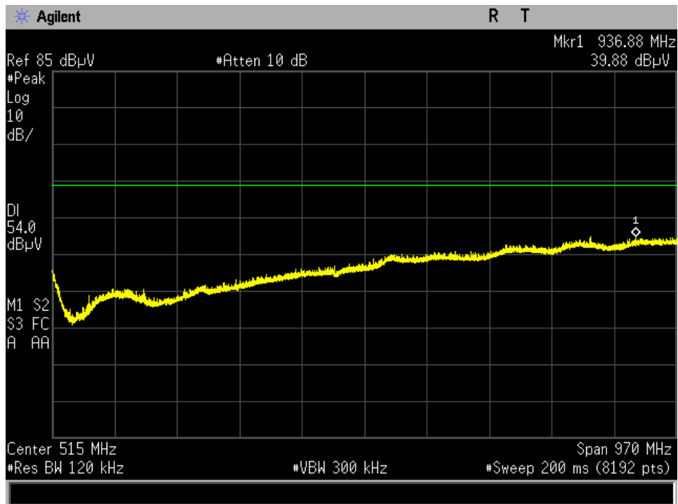
30 MHz-1GHz High Channel outside antenna
