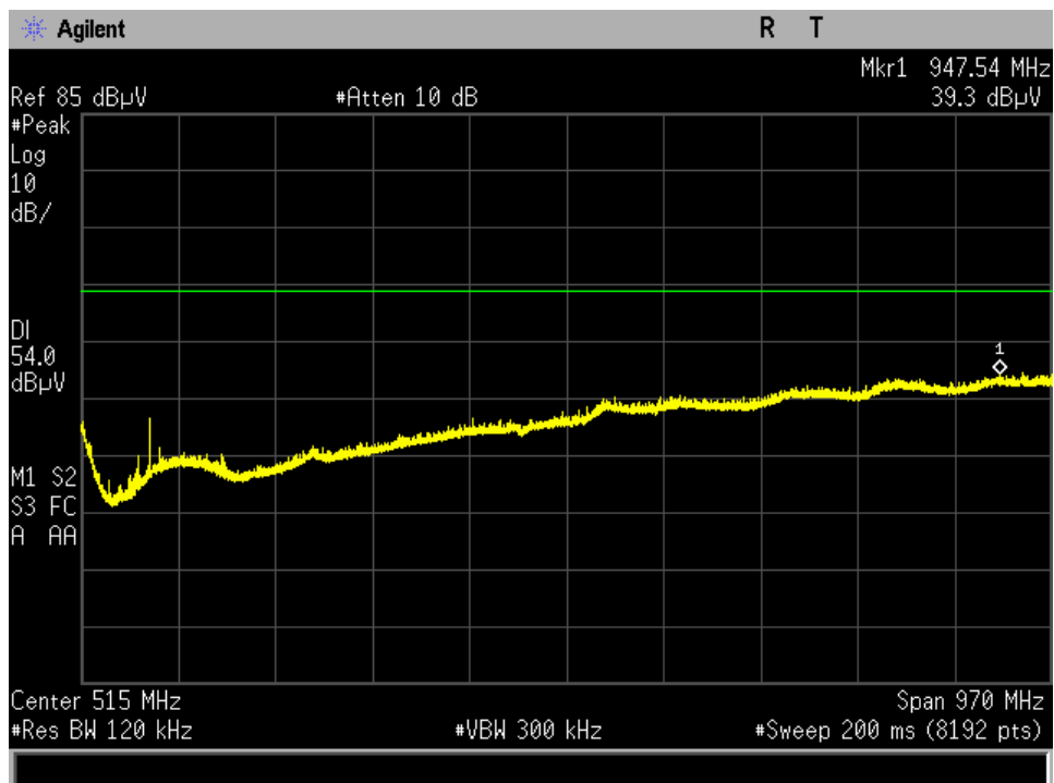
30 MHz-1GHz low Channel outside antenna
