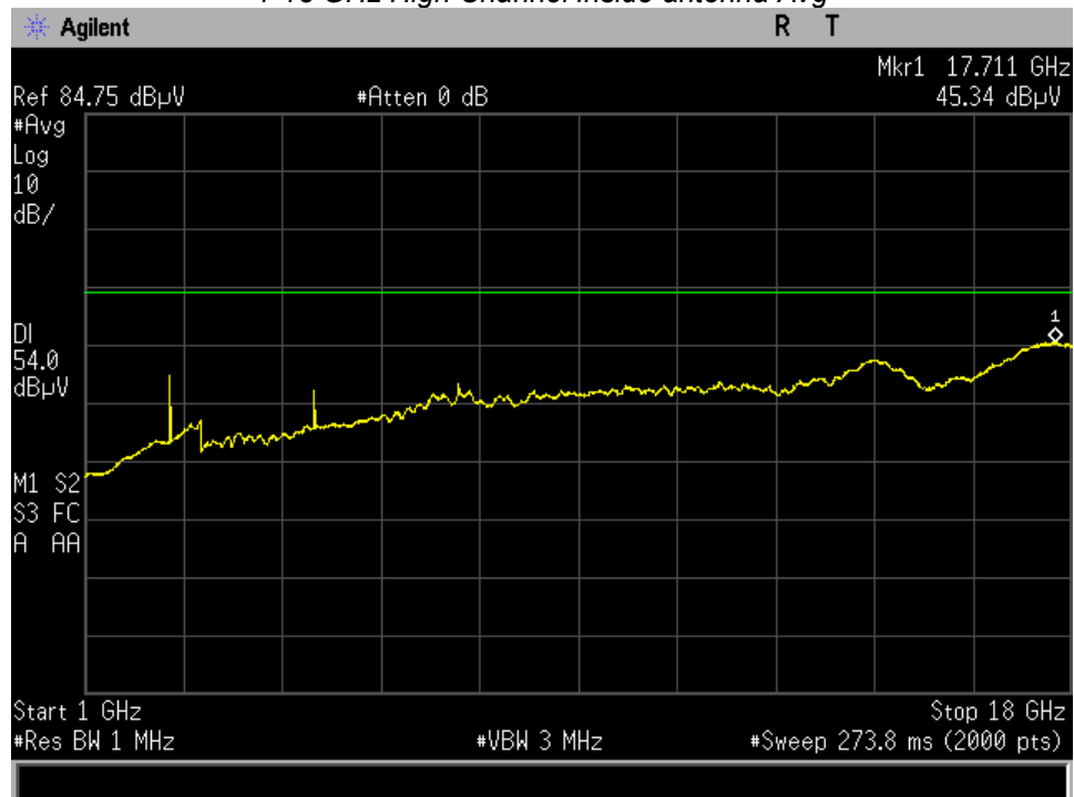
1-18 GHz High Channel inside antenna Avg
