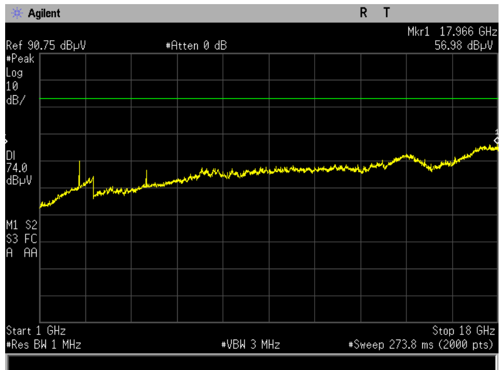
1-18 GHz High Channel inside antenna Peak
