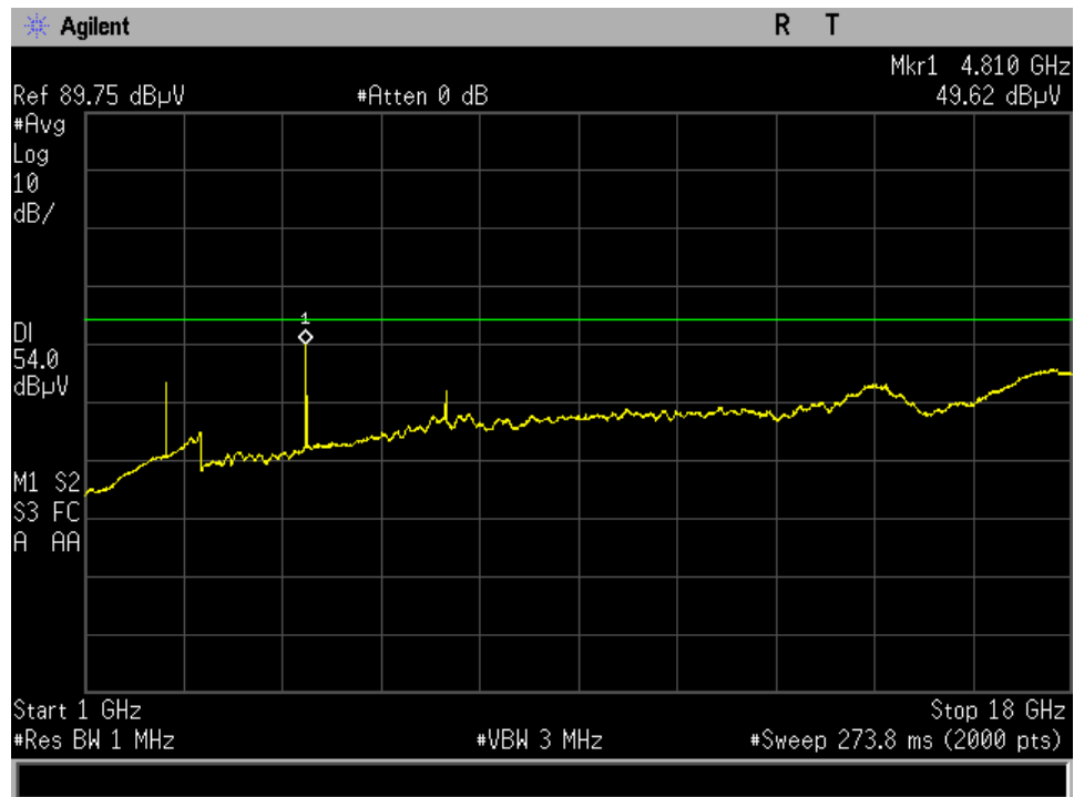
1-18 GHz Low Channel outside antenna Peak
