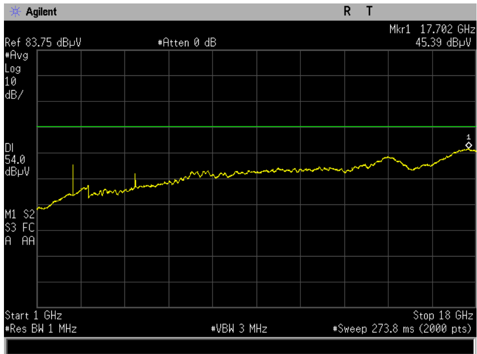
1-18 GHz Low Channel inside antenna Peak
