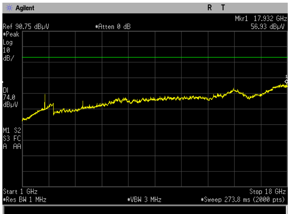
1-18 GHz Middle Channel inside antenna Peak
