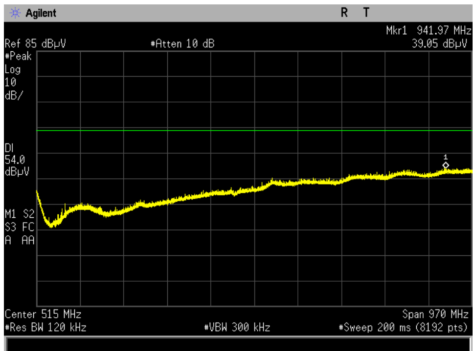
30 MHz-1GHz Mid Channel outside antenna
