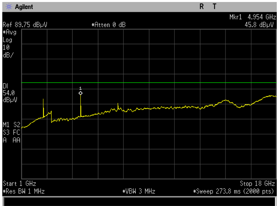
1-18 GHz High Channel outside antenna Peak
