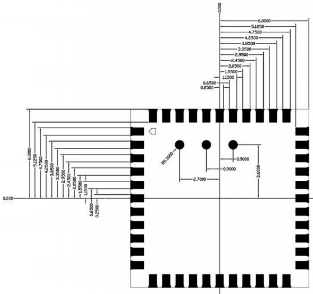
< TOP VIEW >
