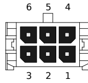
Figure 2.12: MICROFIT 3.0 430450600
