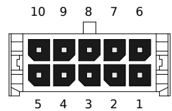
Figure 2.14: MICROFIT 3.0 430451000
