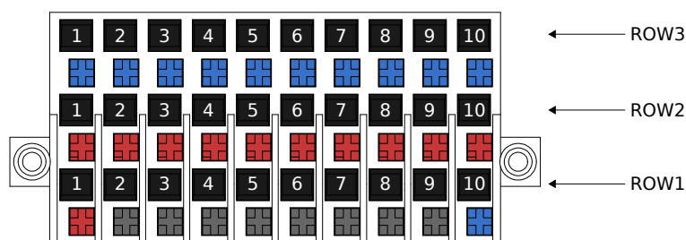
Figure 2.16: WEIDMULLER 1779920000
