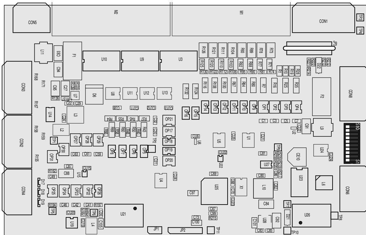
Figure 2.19: dip-switch position
