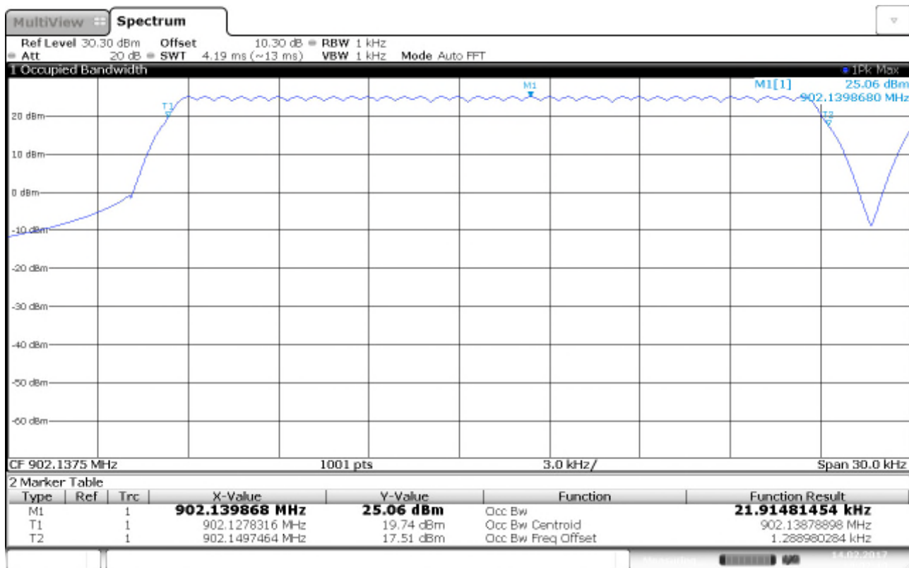
99% Bandwidth – ch902.1375MHz
