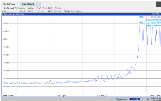
Frequency hopping, Lower Band Edge, Peak
