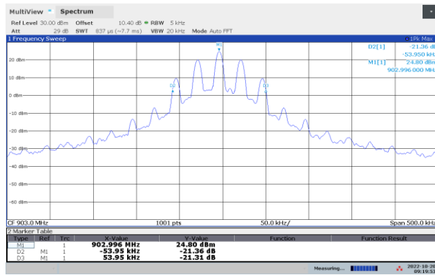
20dB Bandwidth 903 MHz, GFSK
