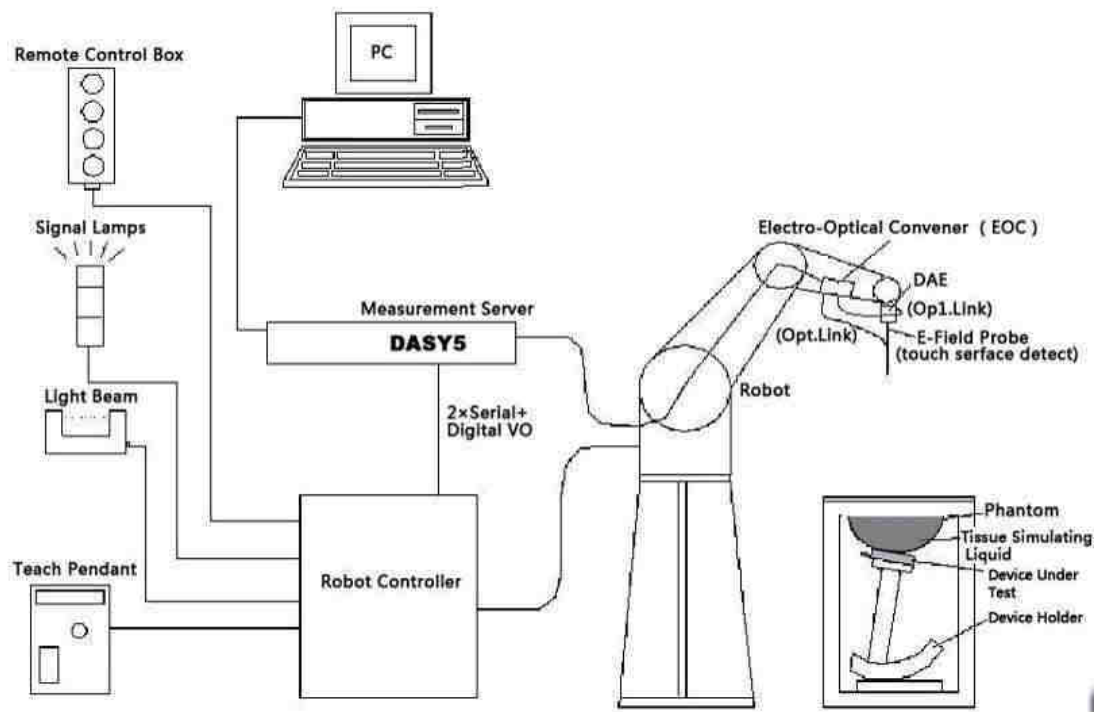
Picture 1. SAR Lab Test Measurement Set-up
