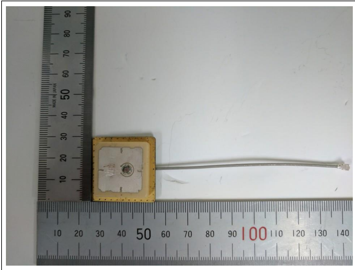
&lt;Antenna 3 - KSA-SP921MS25P20P4B &gt;
