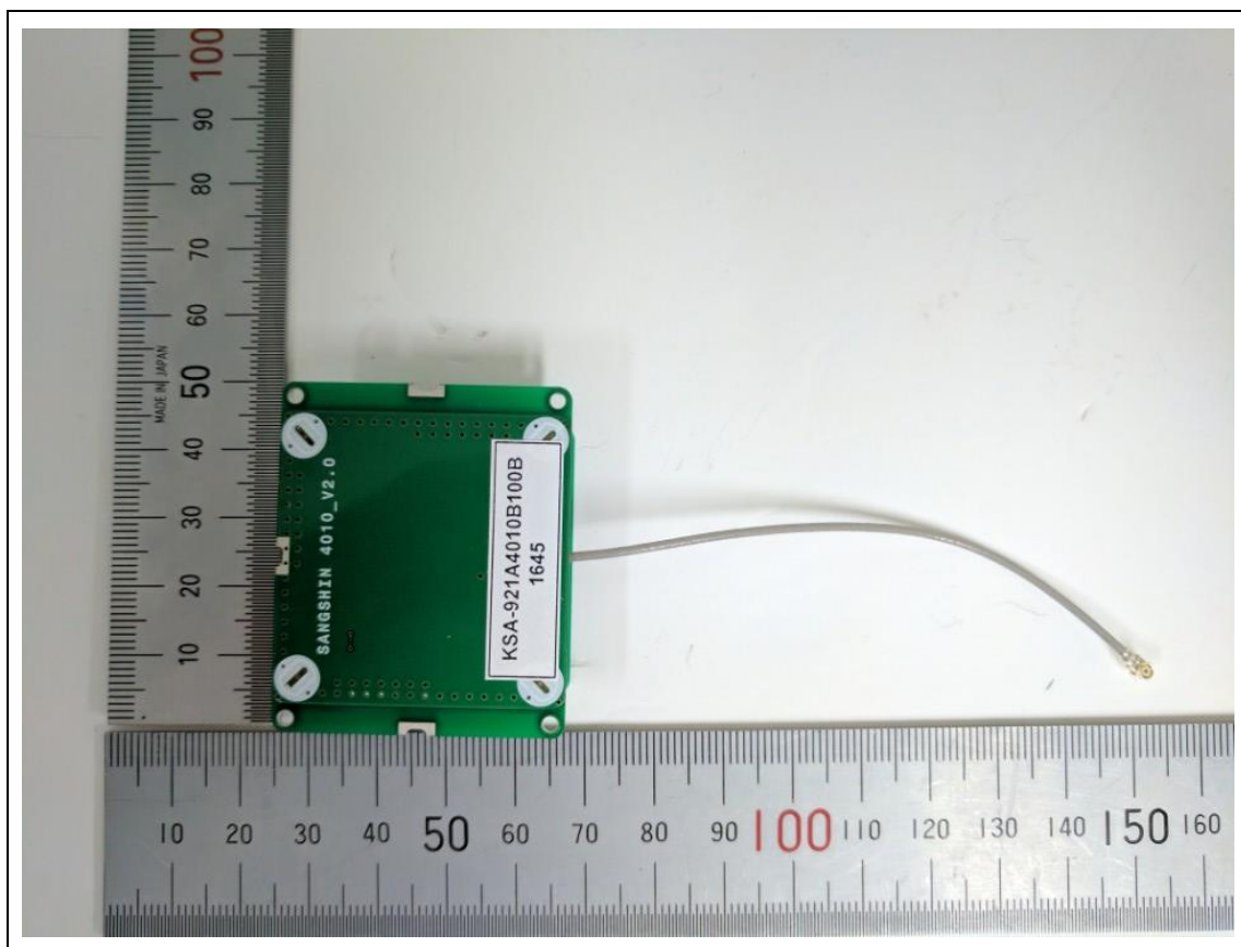
&lt;Antenna 2 - KSA-921A4010B100B &gt;
