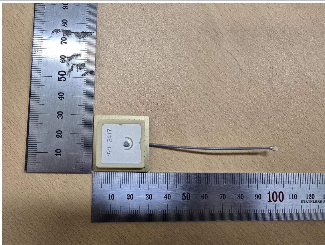
Antenna 2 (M/N: KSA-A921MS25A30C80)
