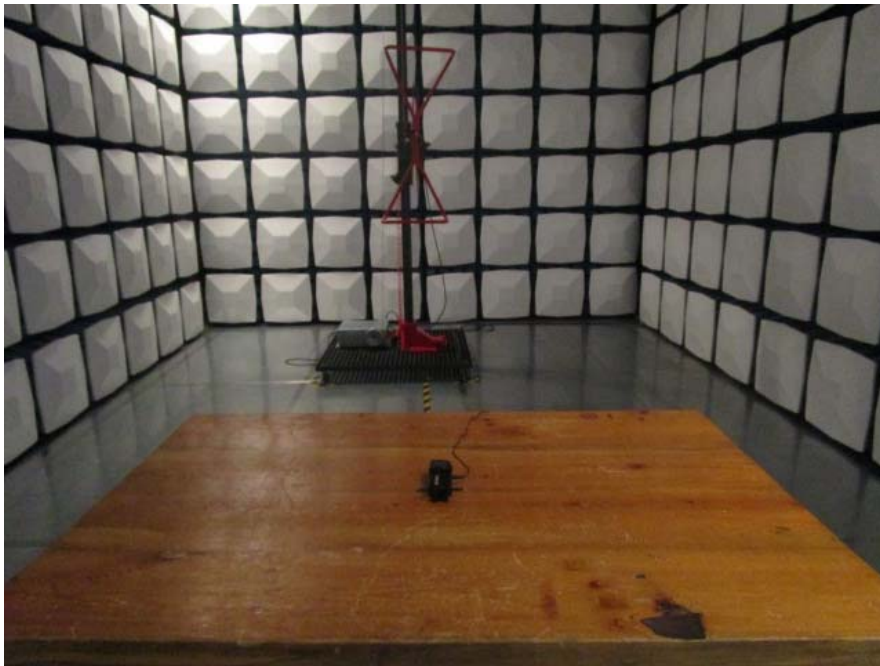
Radiated Emission (Below 1GHz Distance 3m)
