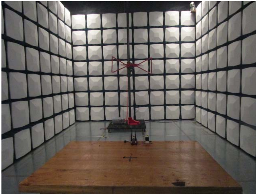
Radiated Emission- Below 1 GHz View-Front View
