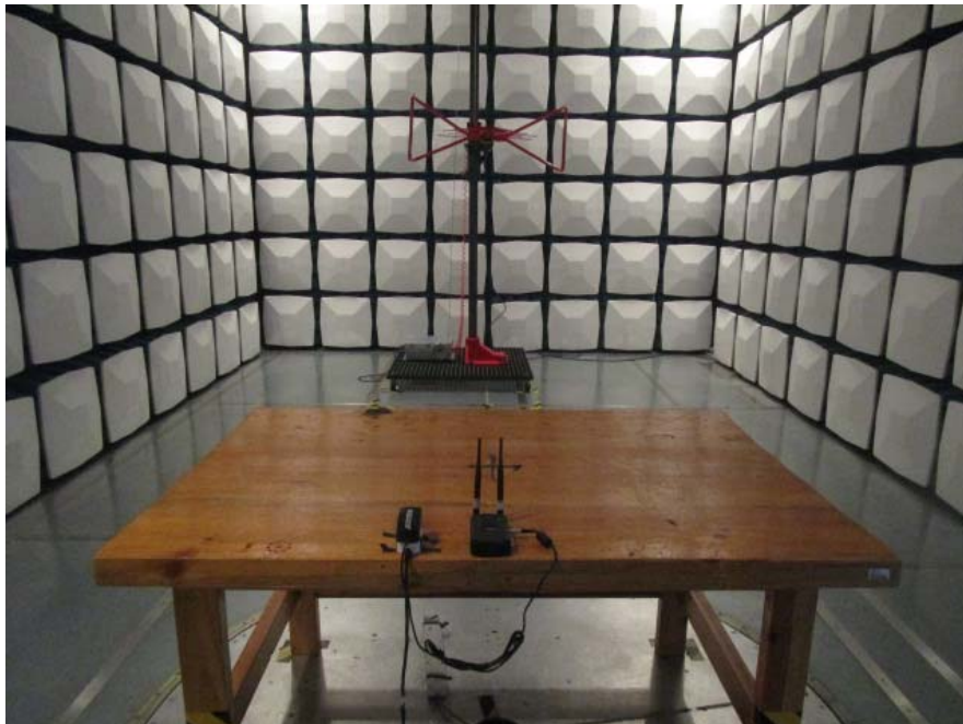
Radiated Emission- Below 1 GHz View-Back View
