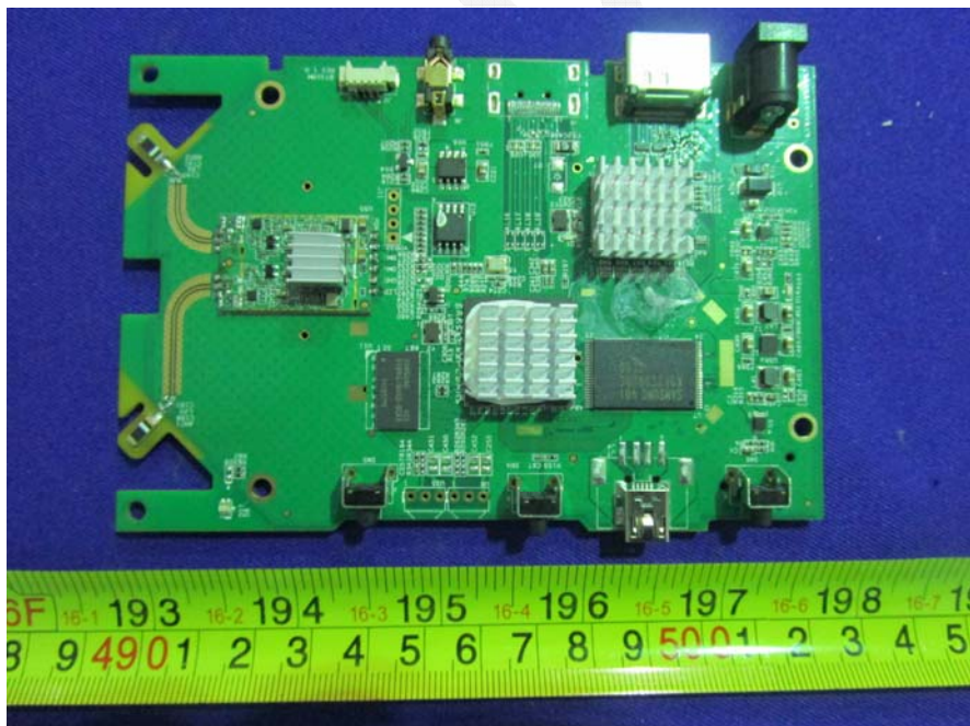
EUT –Main Board With Heatsink View
