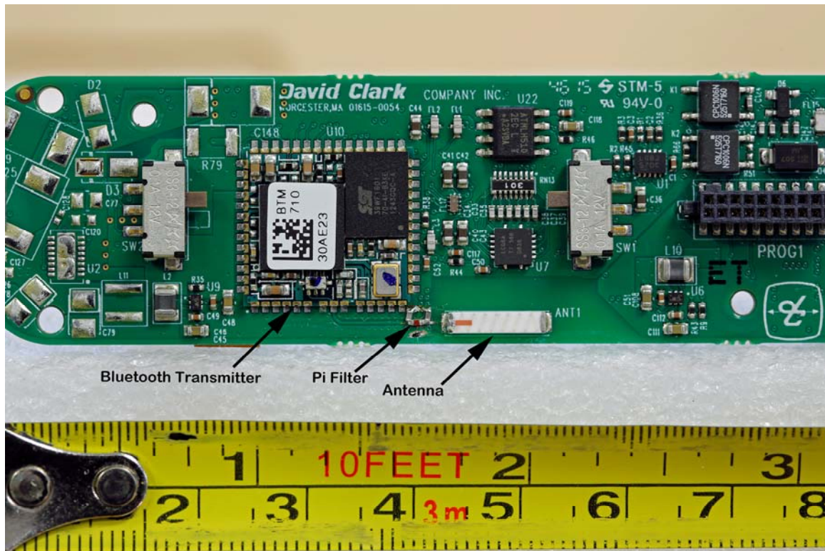
Rear Module – Labeled
