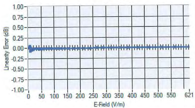
Linearity
