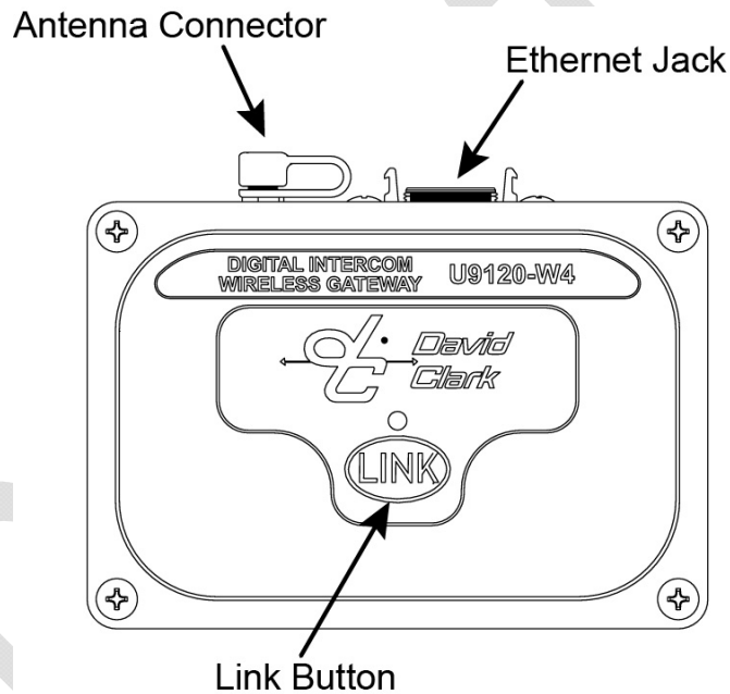
Figure 8.2 Wireless Gateway
