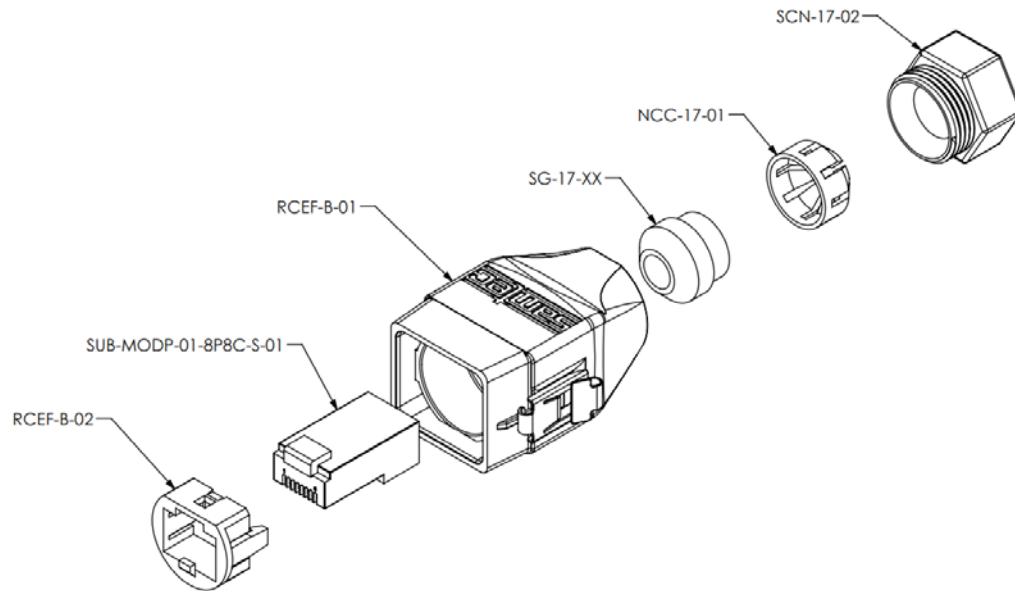
Figure 4.2 Waterproof connector assembly
