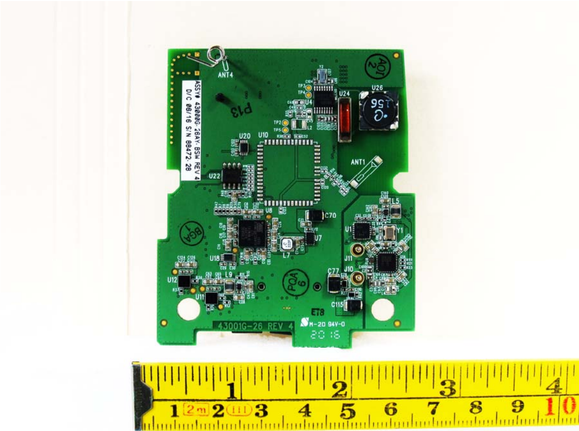
PCB Back
