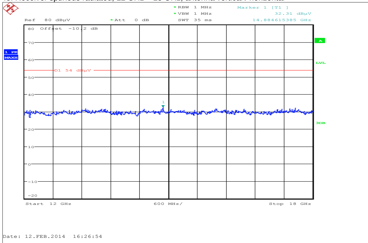
Plot 48: Receiver spurious radiated, 12 GHz – 18 GHz, antenna vertical / horizontal
