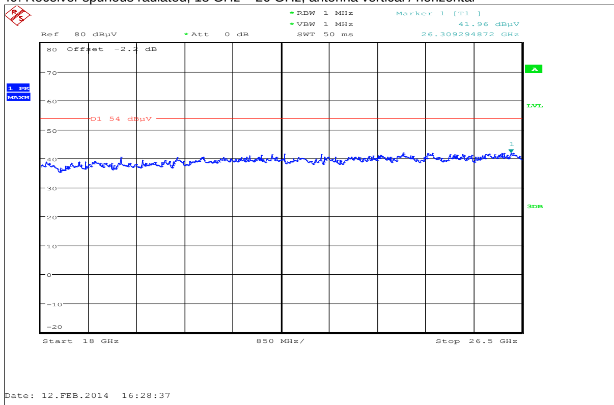
Plot 49: Receiver spurious radiated, 18 GHz – 26 GHz, antenna vertical / horizontal
