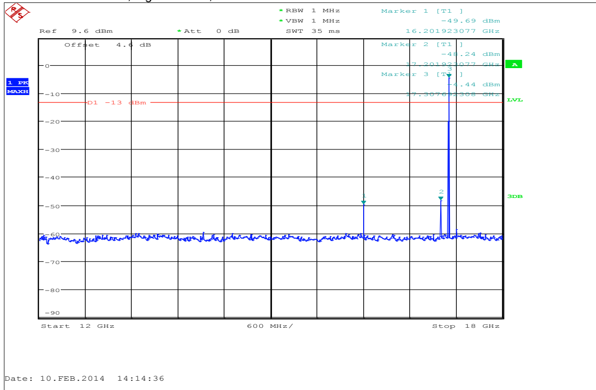
Plot 30: 12 GHz – 18 GHz, high channel, antenna vertical / horizontal
