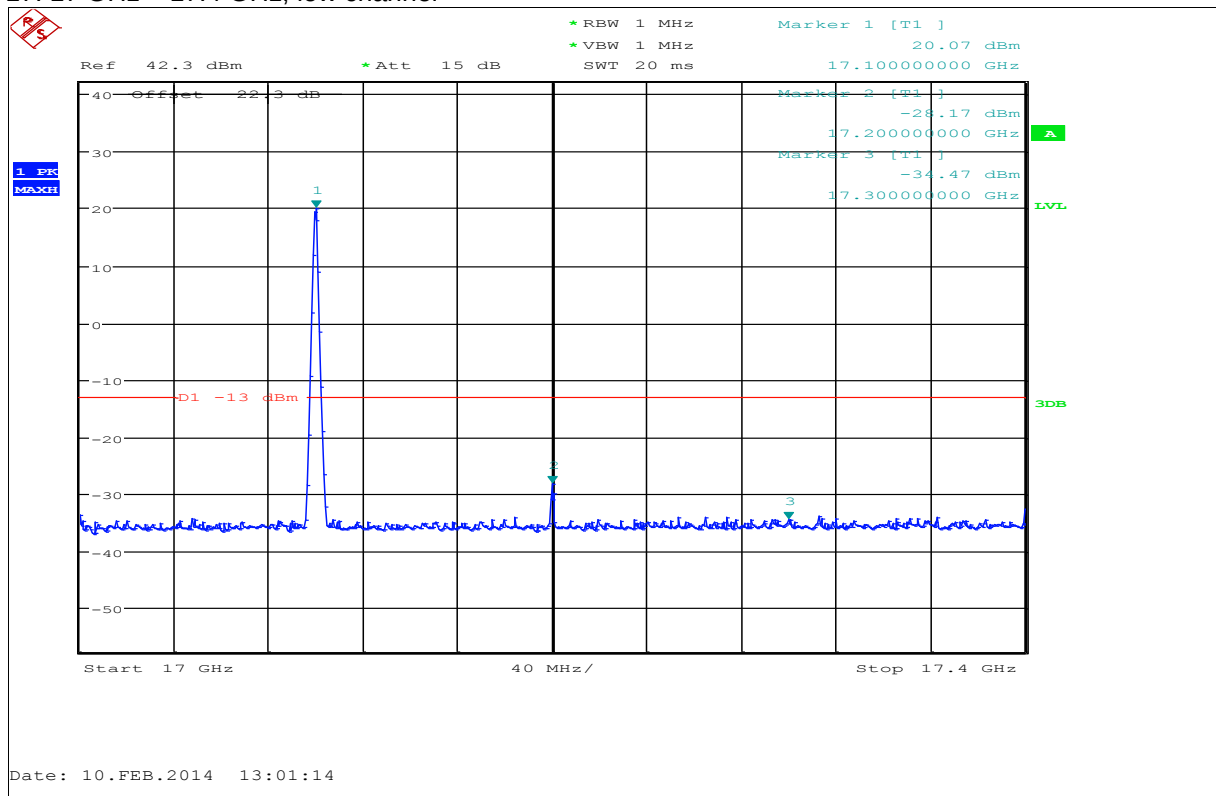
Plot 17: 17 GHz – 17.4 GHz, low channel
