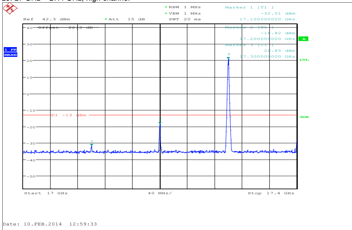
Plot 19: 17 GHz – 17.4 GHz, high channel
