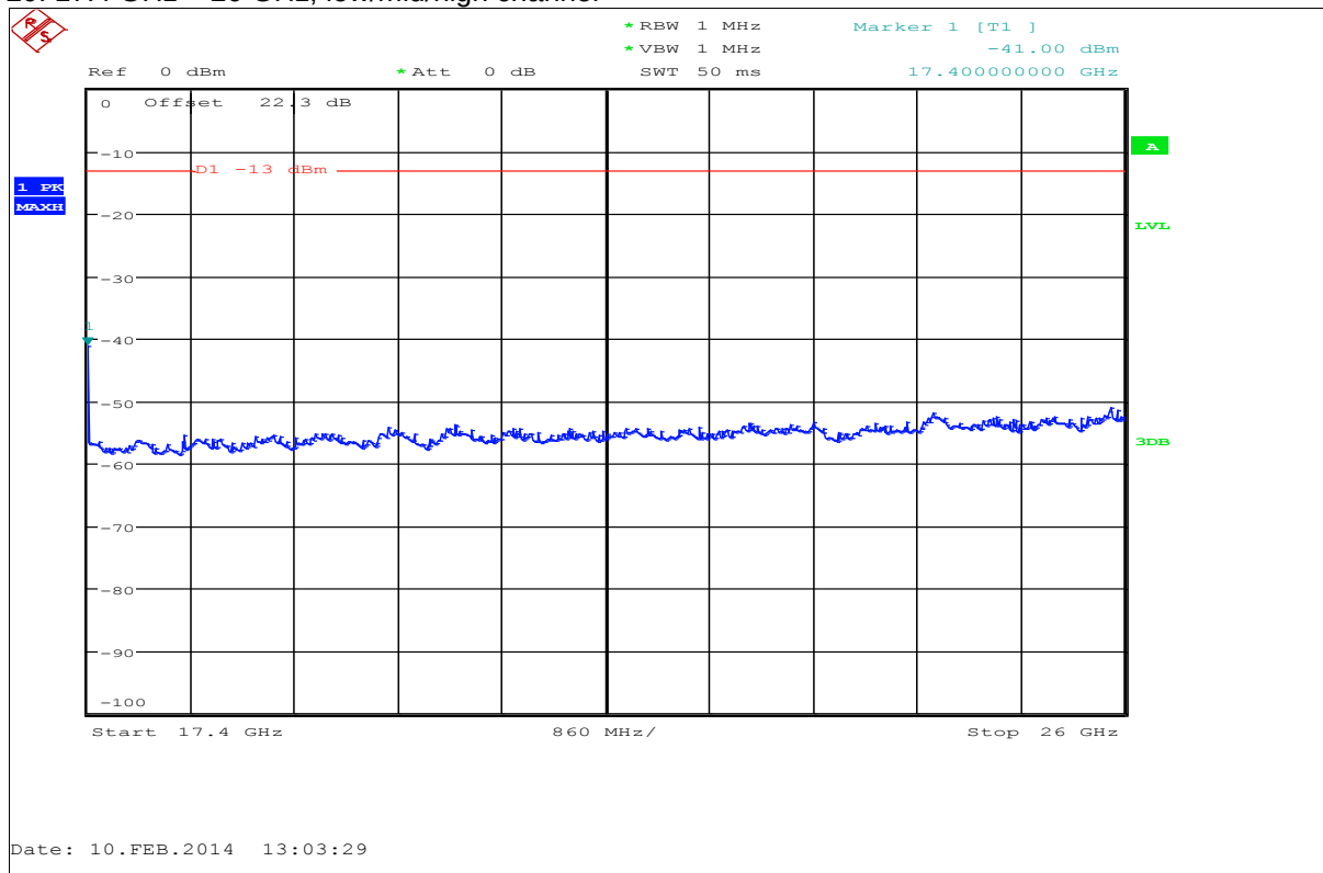
Plot 20: 17.4 GHz – 26 GHz, low/mid/high channel
