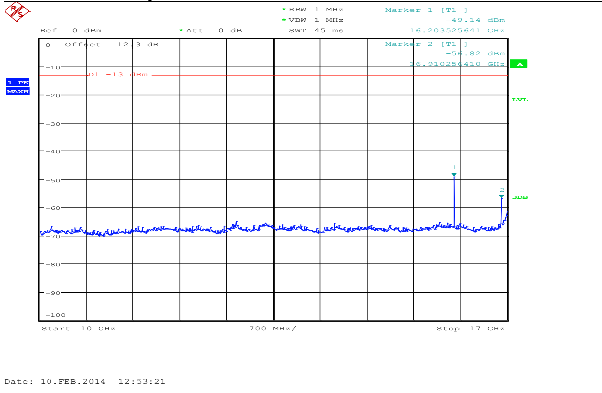
Plot 16: 10 GHz – 17 GHz, high channel
