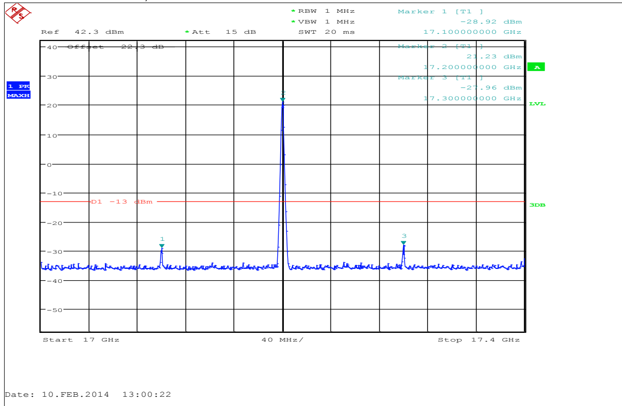
Plot 18: 17 GHz – 17.4 GHz, mid channel
