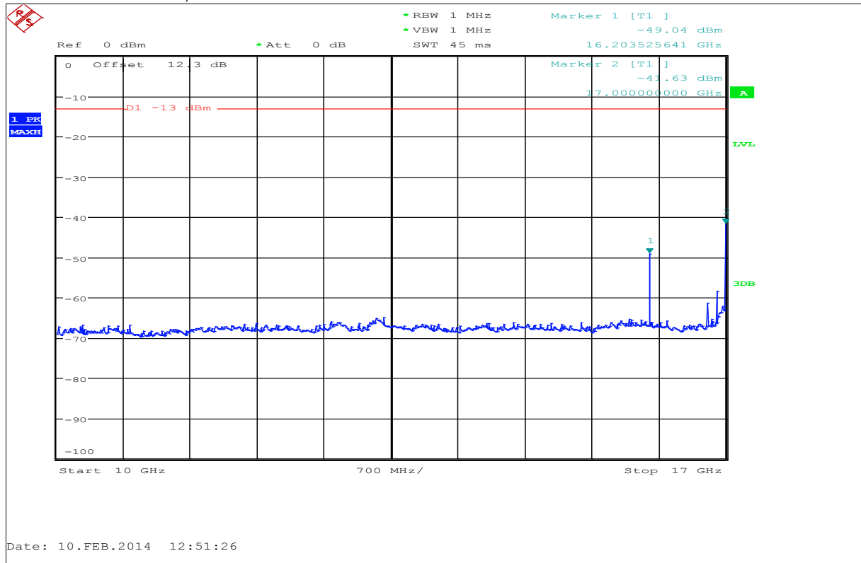
Plot 14: 10 GHz – 17 GHz, low channel
