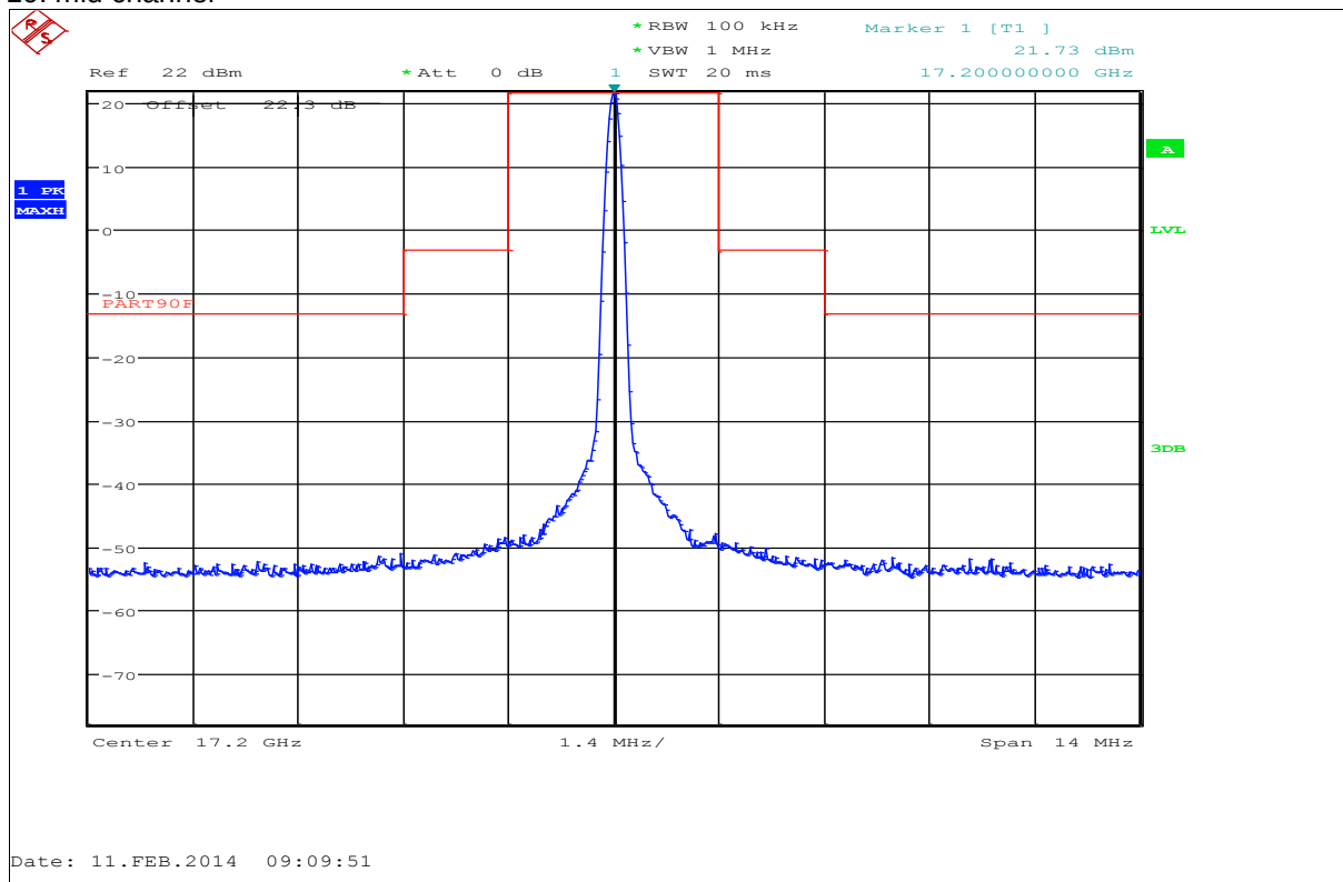
Plot 10: mid channel
