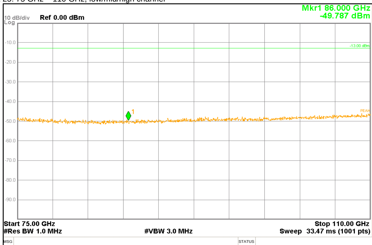
Plot 25: 75 GHz – 110 GHz, low/mid/high channel
