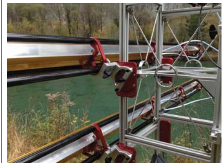
Elevation Adjustment
