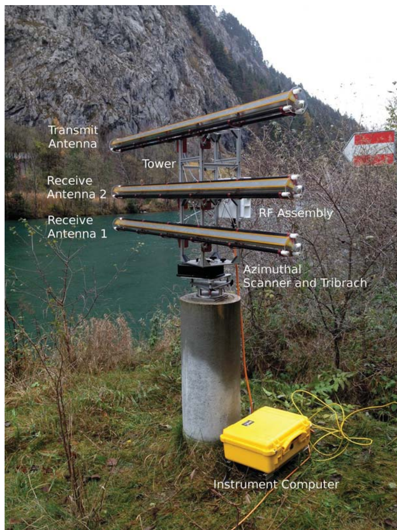
GPRI Radar on Pedestal
