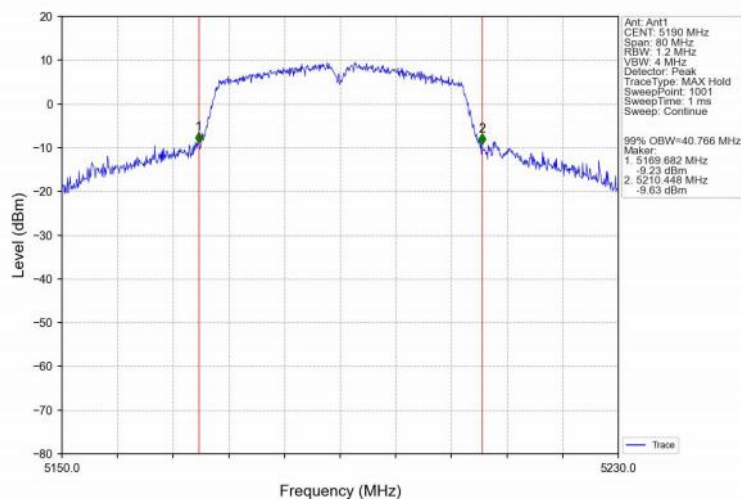
802.11ac(VHT40)_LCH_5190MHz_Ant1_NTNV
