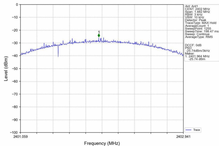
2M_LCH_2402MHz_Ant1_NTNV
