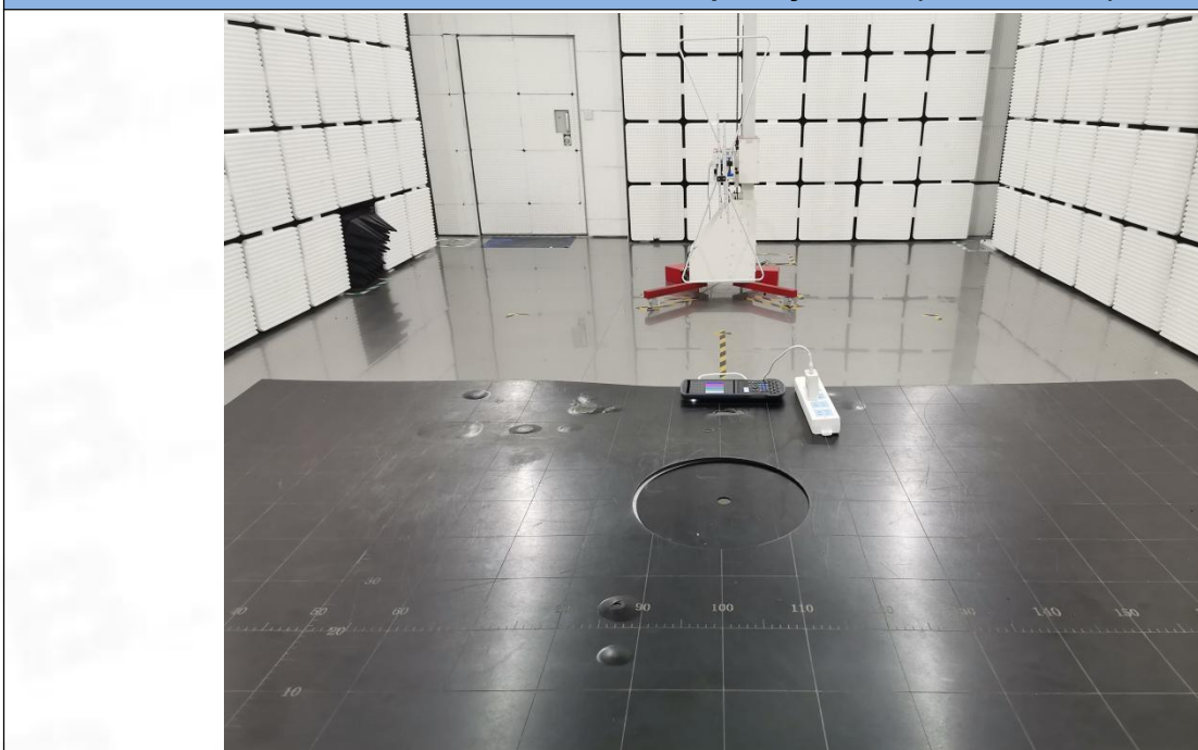
Emissions in restricted frequency bands (30MHz-1GHz)
