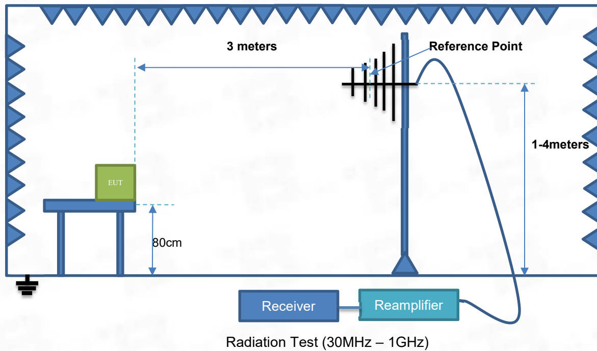
Test Setup 1
