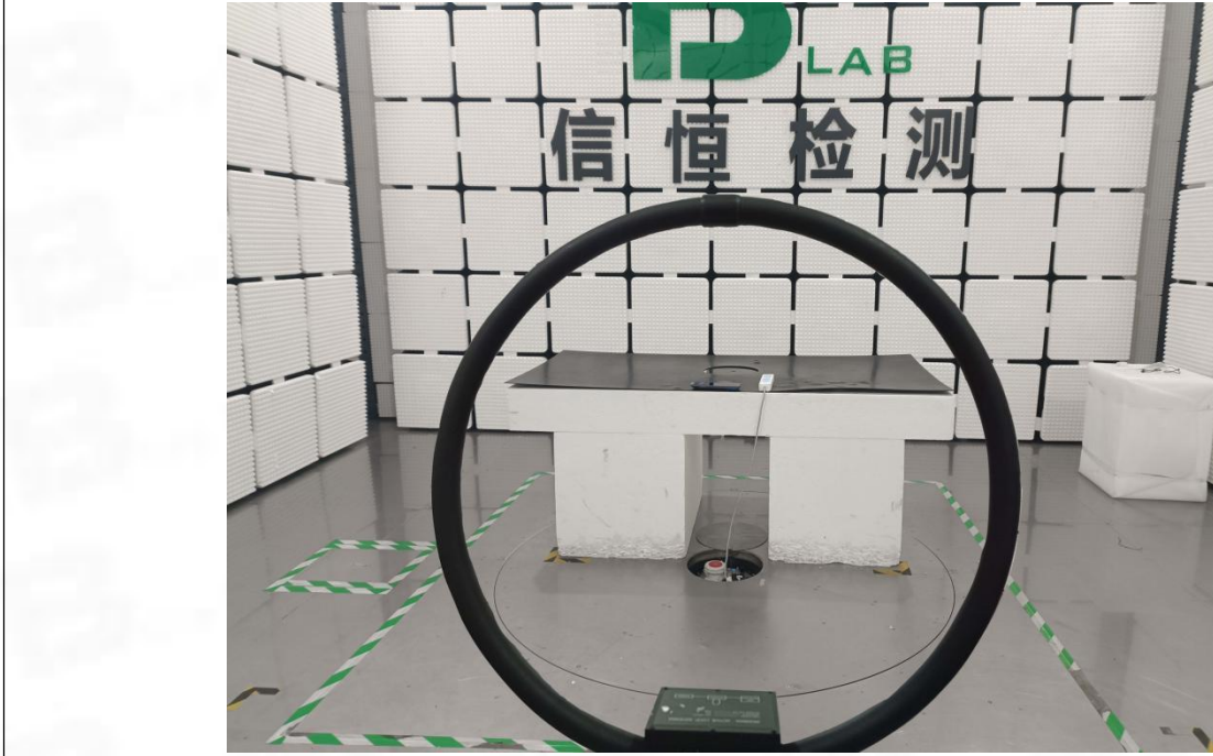
Emissions in restricted frequency bands (9KHz – 30MHz)
