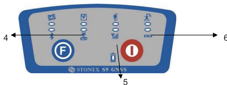
Fig. 2.19 - S9III PLUS summary of data-link led
