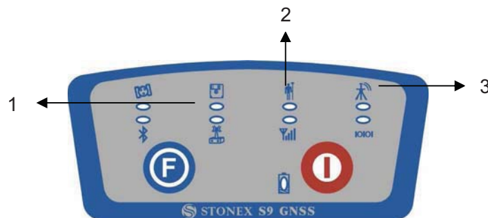
Fig. 2.18 - S9III PLUS summary of working mode led
