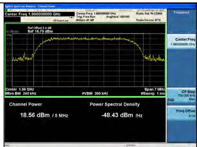
PWR-Band2-QPSK-Mid CH
