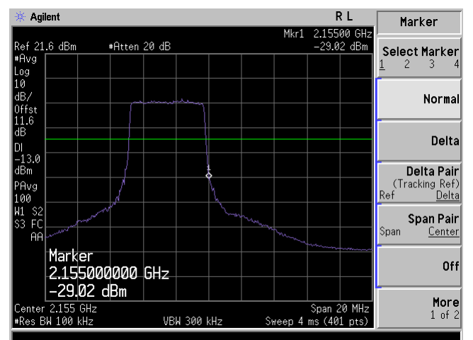
BandEdge-LTE-Band4-5MHz-64QAM-High
