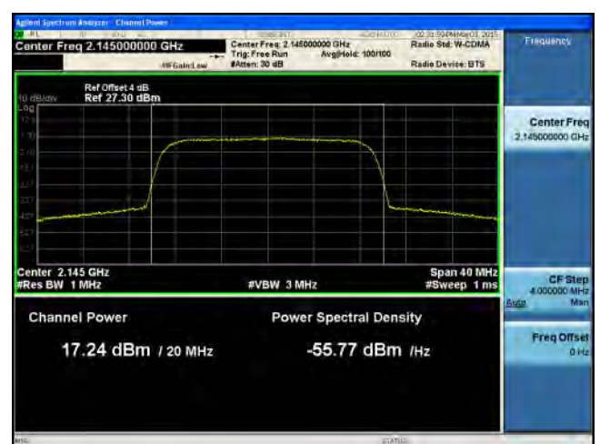
PWR-Band4-16QAM-20M BW-High CH-Port2
