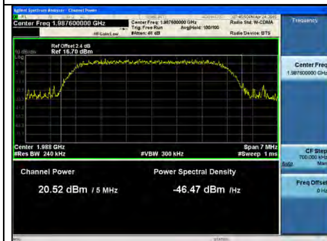
PWR-Band2-QPSK--High CH
