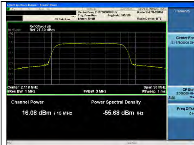
PWR-Band4-16QAM-15M BW-Low CH-Port1
