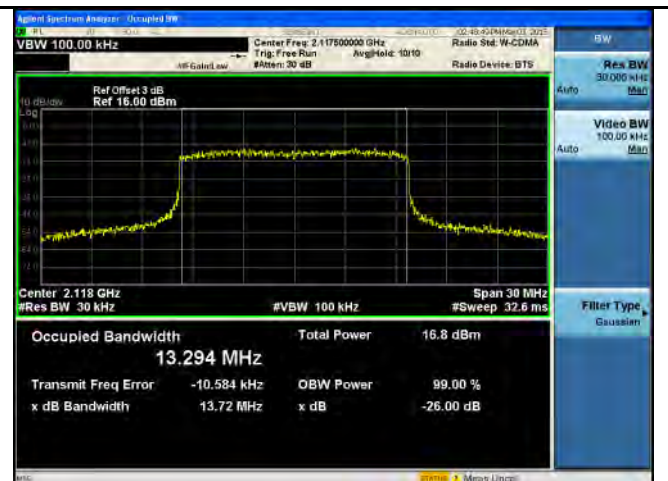
OBW-Band4-15M BW-Low- 16QAM
