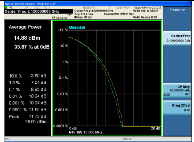
PK-AV-Ratio-Band4-16QAM-20M BW-Low
