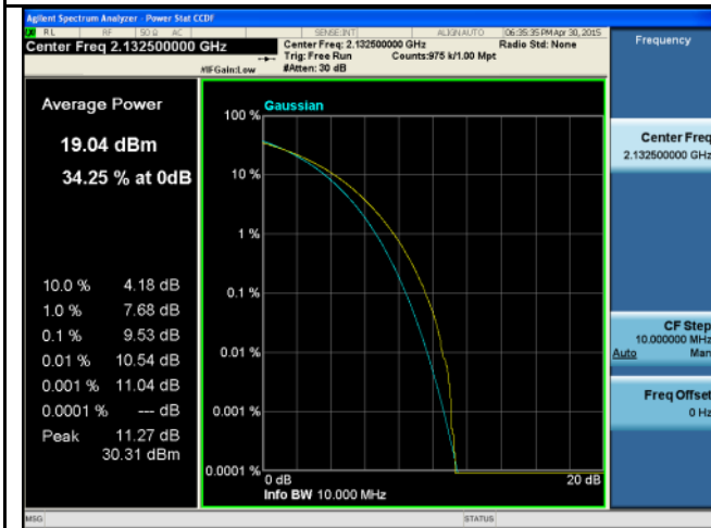
PK-AV-Ratio-Band4-QPSK-5M BW-Mid
