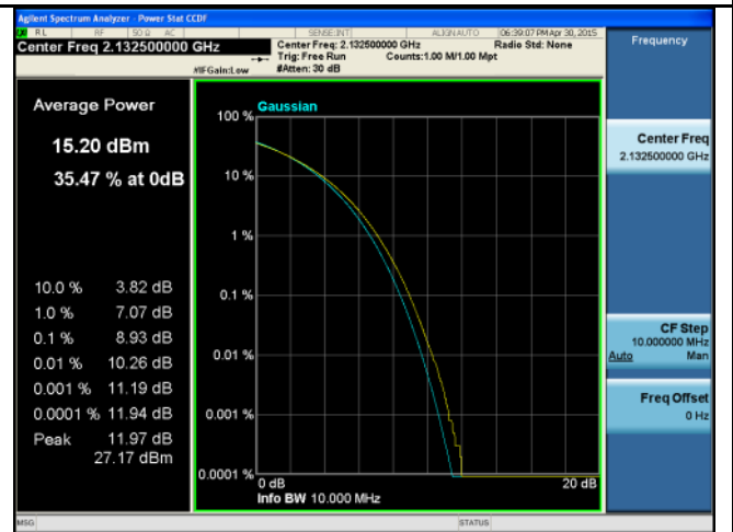
PK-AV-Ratio-Band4-QPSK-10M BW-Mid
