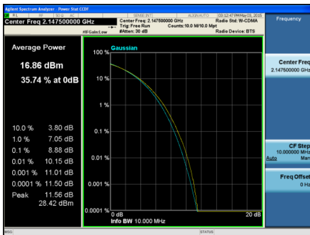
PK-AV-Ratio-Band4-16QAM-15M BW-High
