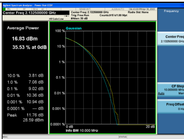
PK-AV-Ratio-Band4-64QAM-15M BW-Mid
