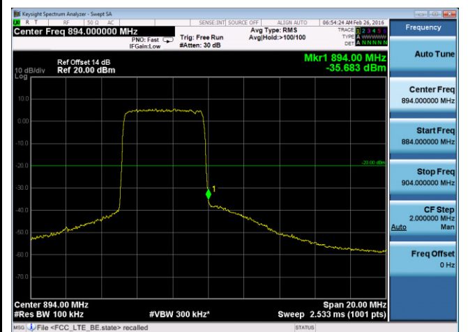
BandEdge-LTE- Band5-5MHz -64QAM-High
