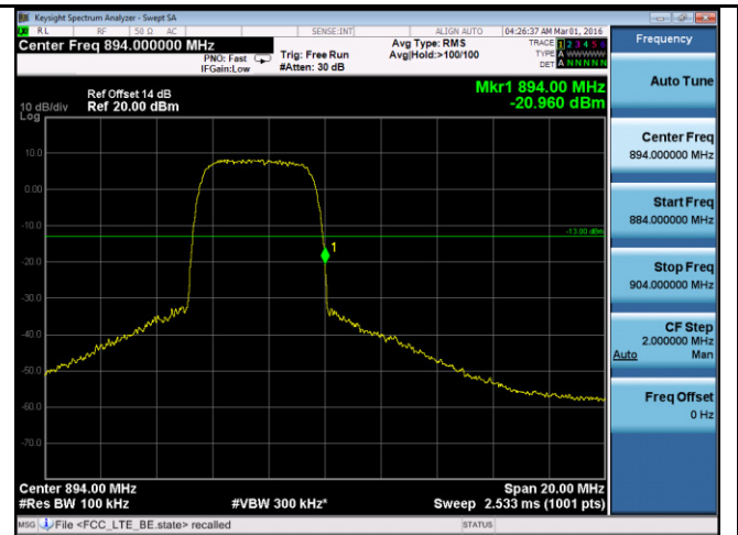
BandEdge-WCDMA- Band5-5MHz-QPSK-High
