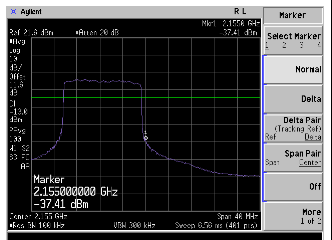
BandEdge-LTE-Band4-15MHz-64QAM-High
