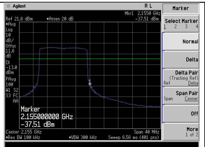
BandEdge-LTE-Band4-15MHz-QPSK-High
