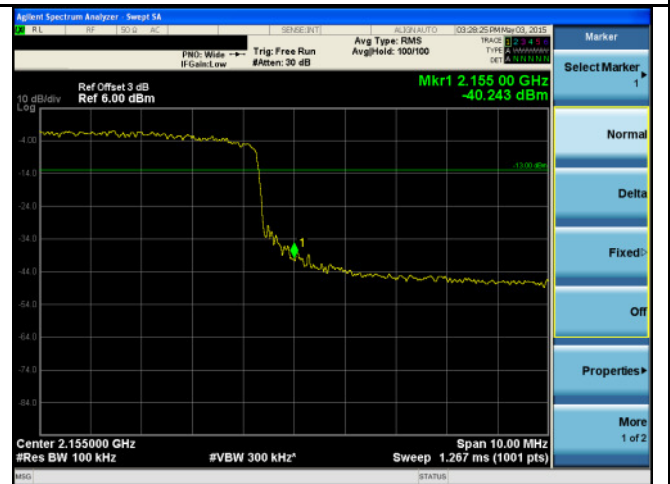
BandEdge-LTE-Band4-15MHz-16QAM-High
