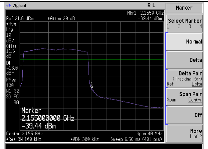
BandEdge-LTE-Band4-20MHz-QPSK-High
