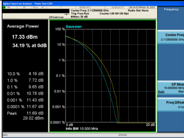
PK-AV-Ratio-Band4-64QAM-5M BW-Low
