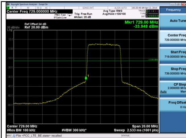
BandEdge-LTE- Band12-5MHz-64QAM -Low
