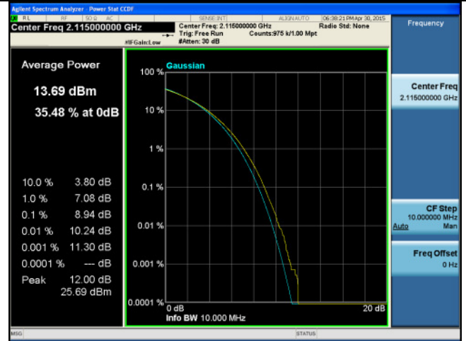
PK-AV-Ratio-Band4-64QAM-10M BW-Low
