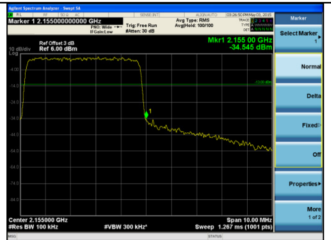
BandEdge-LTE-Band4-5MHz-16QAM-High
