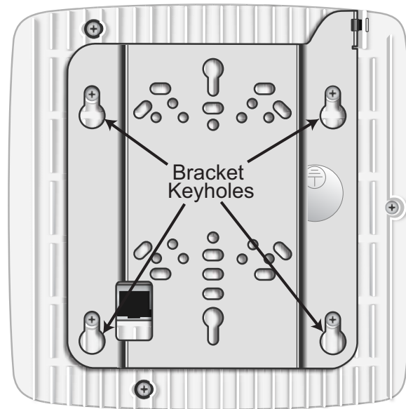
Figure 11 Radio Node Slides into Mount Bracket
