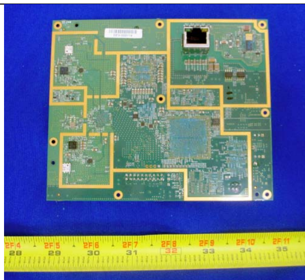
Main Board – Bottom View
