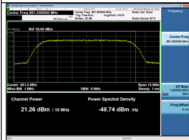
PWR- Band5-64QAM-10M BW-Mid CH-Port1
