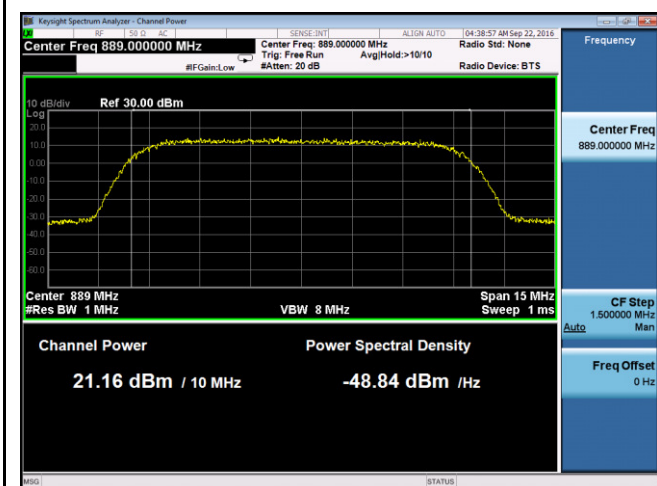
PWR- Band5-64QAM-10M BW-High CH-Port1
