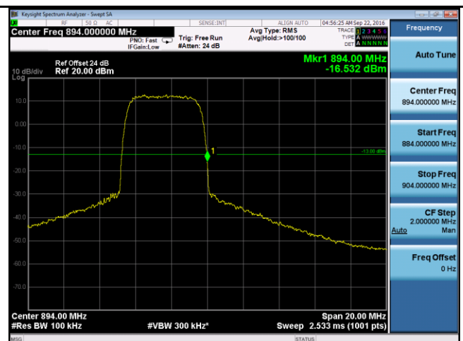
BandEdge-WCDMA- Band5-5MHz-QPSK-High
