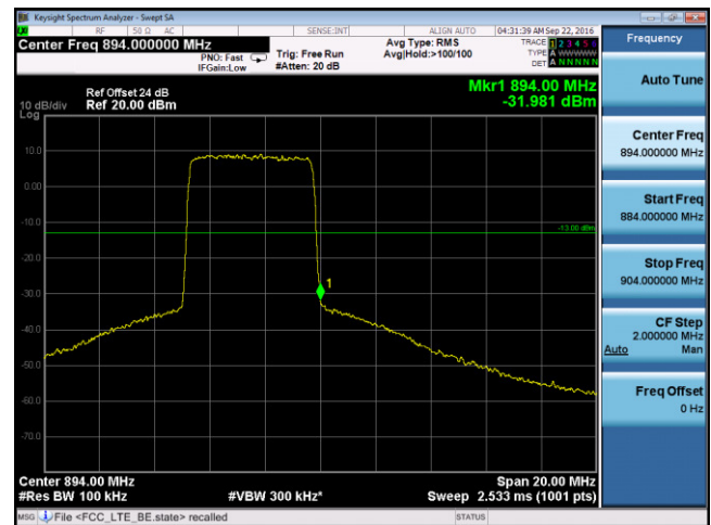
BandEdge-LTE- Band5-5MHz-64QAM-High
