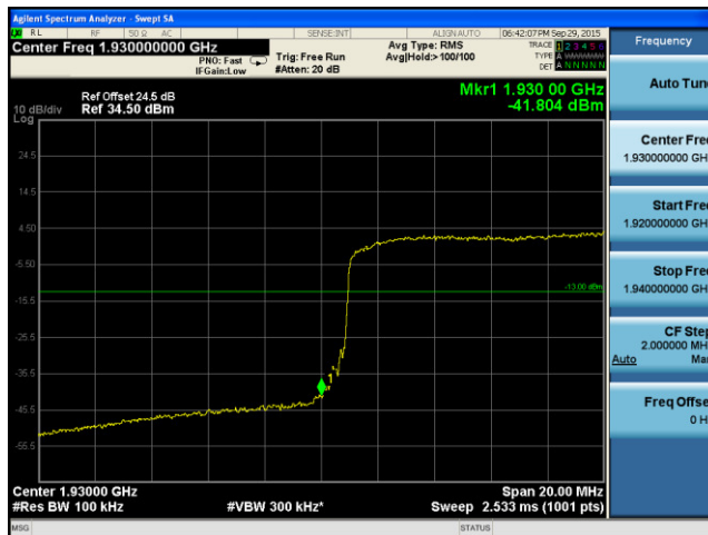
BandEdge-LTE- Band2-20MHz-64QAM-Low
