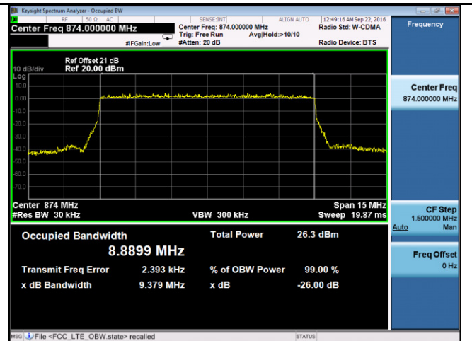
OBW- Band5-10M BW-Low
