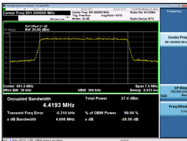
OBW- Band5-5M BW-High
