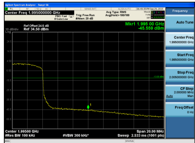
BandEdge-LTE- Band2-20MHz-64QAM-High
