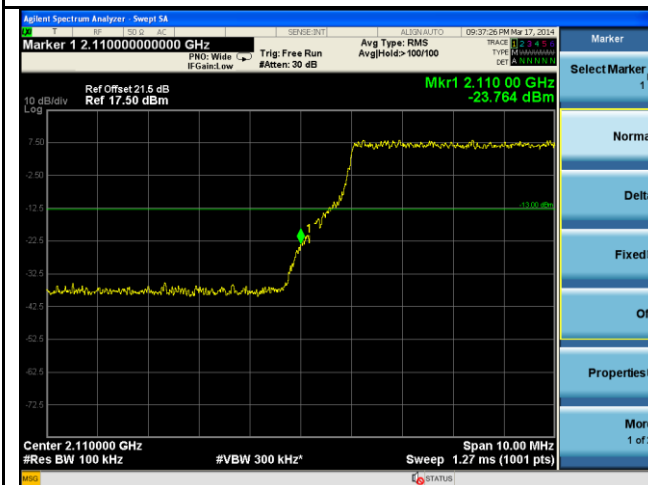
BandEdge-LTE-Band4-20MHz-16QAM-Low
