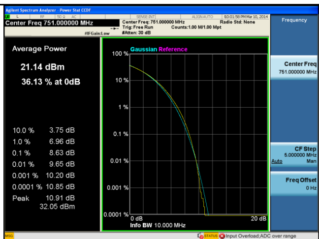
PK-AV-Ratio-Band13-16QAM-10M BW-Mid
