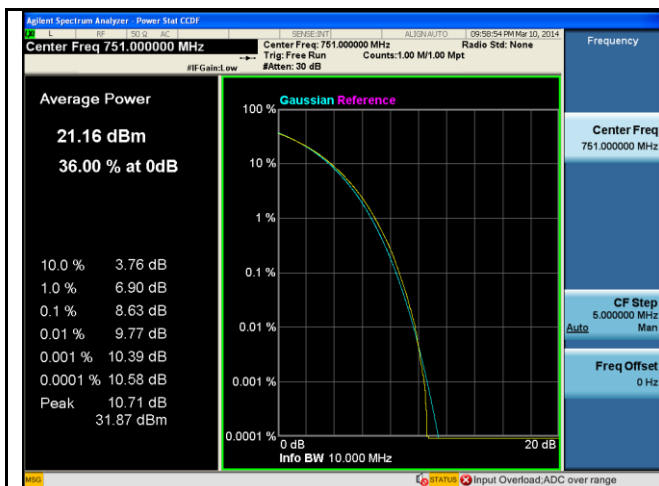
PK-AV-Ratio-Band13-QPSK-10M BW-Mid
