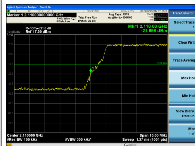
BandEdge-LTE-Band4-20MHz-64QAM-Low
