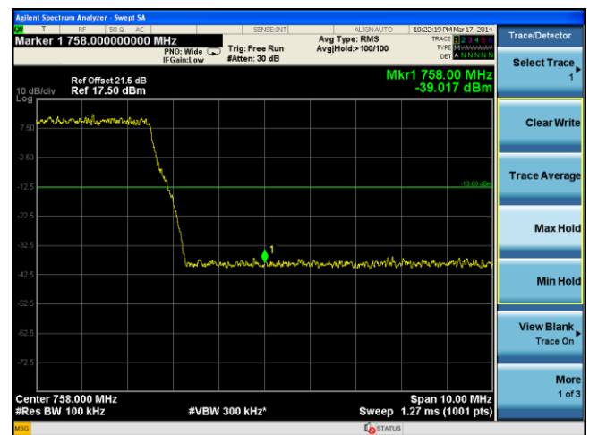
BandEdge-LTE-Band13-10MHz-16QAM-High
