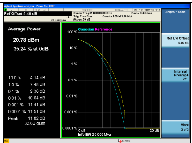
PK-AV-Ratio-Band4-64QAM-20M BW-Low
