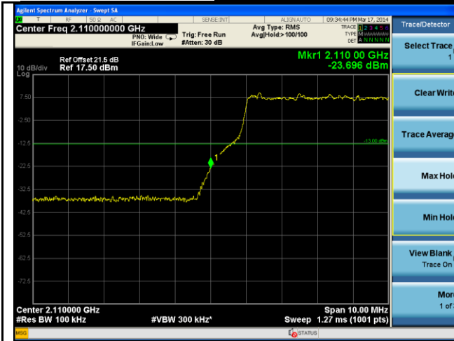
BandEdge-LTE-Band4-20MHz-QPSK-Low
