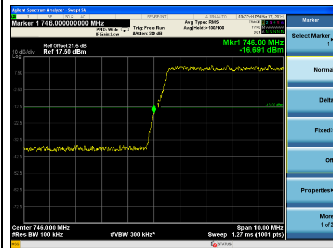
BandEdge-LTE-Band13-10MHz-16QAM-Low
