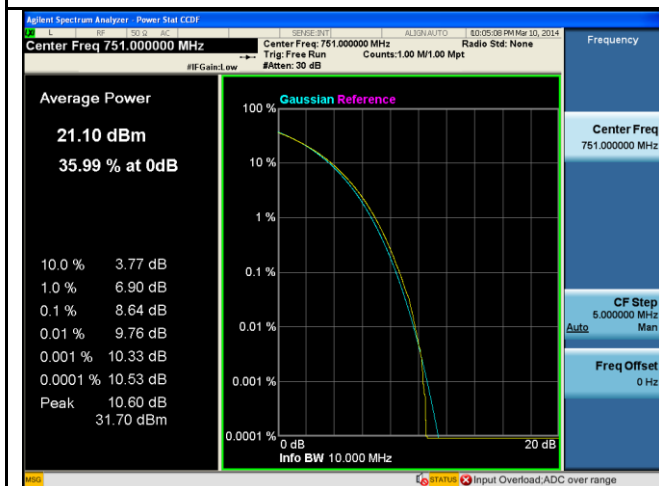
PK-AV-Ratio-Band13-64QAM-10M BW-Mid
