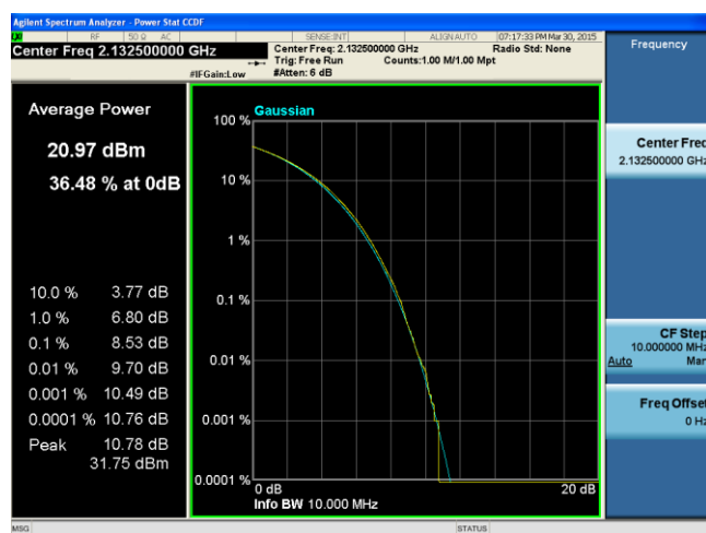
PK-AV-Ratio-Band4-QPSK-15M BW-Mid
