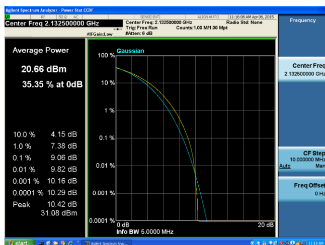
PK-AV-Ratio-Band4-QPSK-5M BW-Mid
