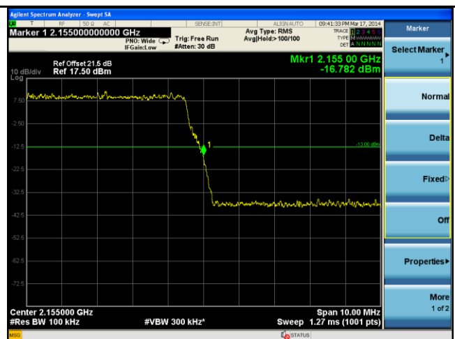
BandEdge-LTE-Band4-10MHz-QPSK-High
