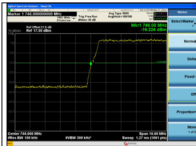
BandEdge-LTE-Band13-10MHz-QPSK-Low
