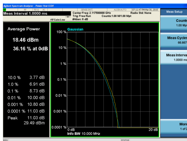
PK-AV-Ratio-Band4-QPSK-15M BW-Low
