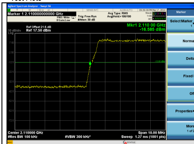
BandEdge-LTE-Band4-10MHz-QPSK-Low
