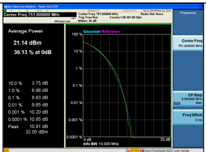
PK-AV-Ratio-Band13-16QAM-10M BW-Mid
