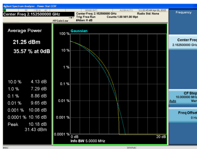
PK-AV-Ratio-Band4-QPSK-5M BW-High
