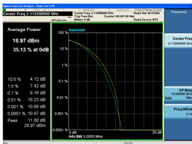
PK-AV-Ratio-Band4-QPSK-5M BW-Low
