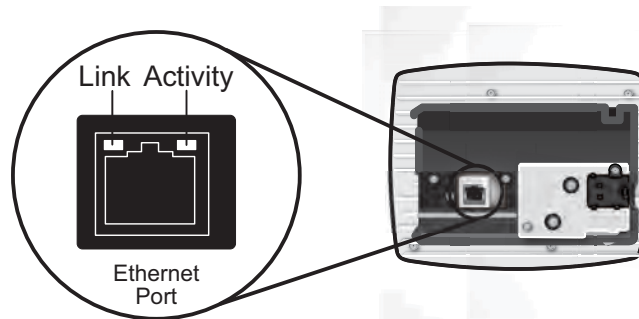
Figure 4 Ethernet Port
