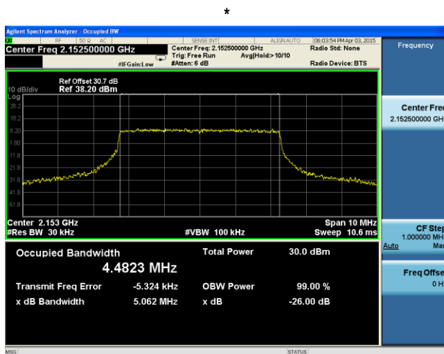
OBW-Band4-5M BW-High
