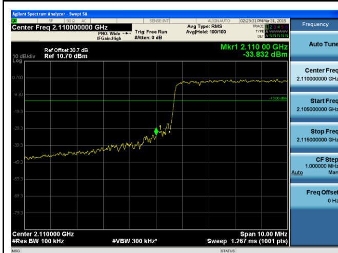
BandEdge-LTE-Band4-15MHz-64QAM-Low
