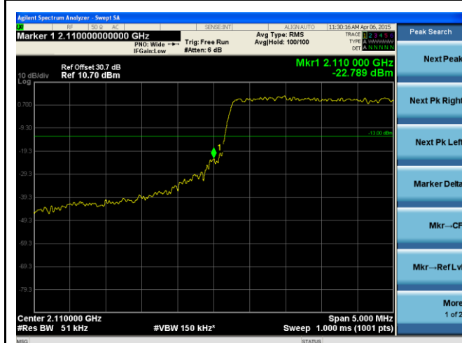
BandEdge-LTE-Band4-5MHz-64QAM-Low
