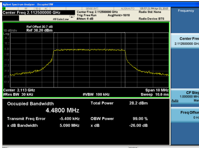
OBW-Band4-5M BW-Low
