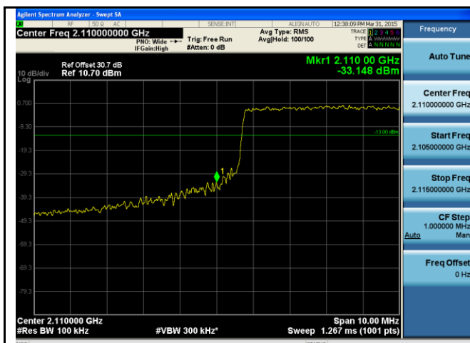
BandEdge-LTE-Band4-15MHz-QPSK-Low
