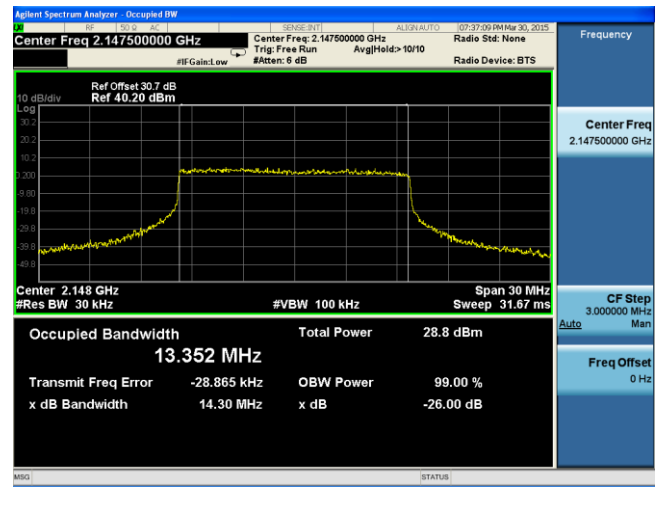
OBW-Band4-15M BW-High
