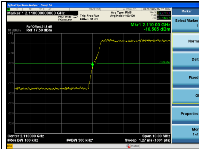
BandEdge-LTE-Band4-10MHz-QPSK-Low
