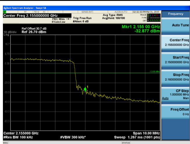
BandEdge-LTE-Band4-15MHz-64QAM-High
