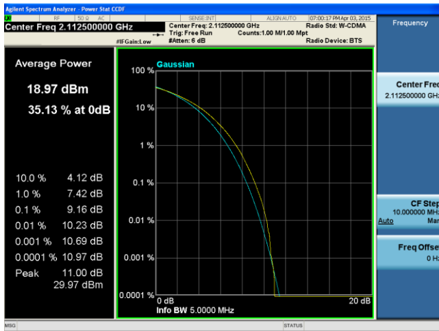
PK-AV-Ratio-Band4-QPSK-5M BW-Low
