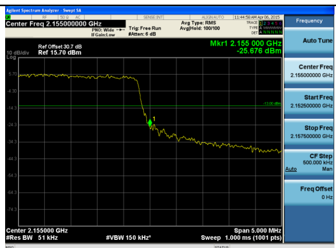
BandEdge-LTE-Band4-5MHz-QPSK-High
