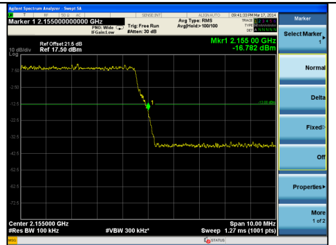
BandEdge-LTE-Band4-10MHz-QPSK-High
