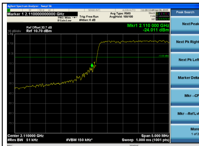
BandEdge-LTE-Band4-5MHz-QPSK-Low
