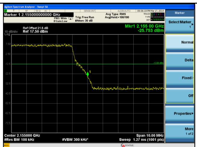
BandEdge-LTE-Band4-20MHz-QPSK-High
