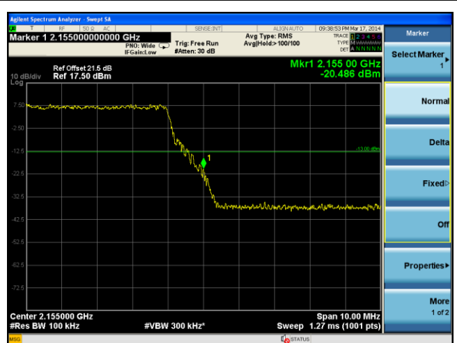
BandEdge-LTE-Band4-20MHz-64QAM-High
