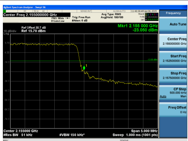
BandEdge-LTE-Band4-5MHz-64QAM-High
