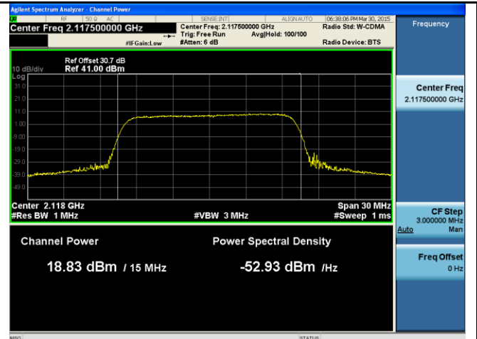
PWR-Band4-QPSK-15M BW-Low CH-Port2
