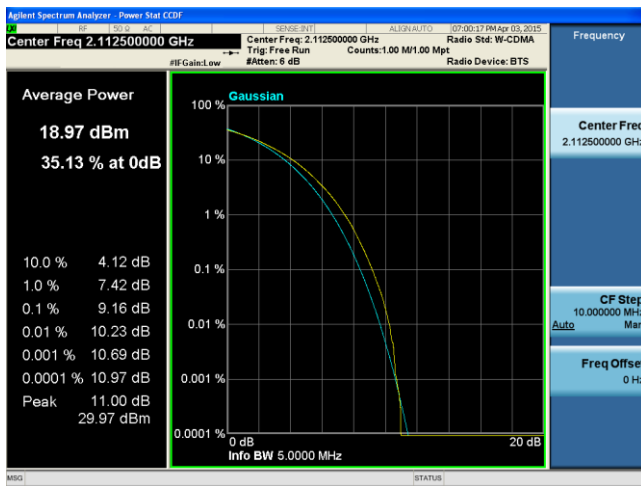
PK-AV-Ratio-Band4-QPSK-5M BW-Low
