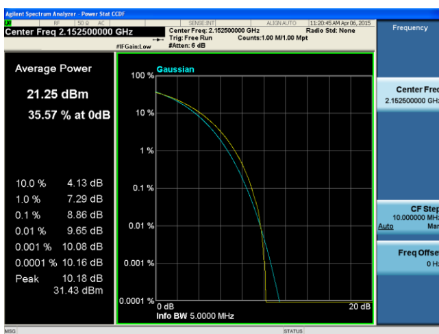
PK-AV-Ratio-Band4-QPSK-5M BW-High
