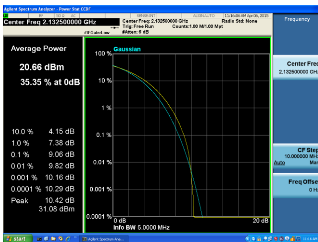
PK-AV-Ratio-Band4-QPSK-5M BW-Mid
