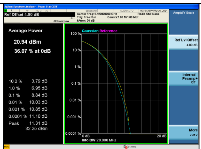
PK-AV-Ratio-Band4-QPSK-20M BW-Low
