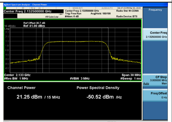
PWR-Band4-QPSK-15M BW-Mid CH-Port2
