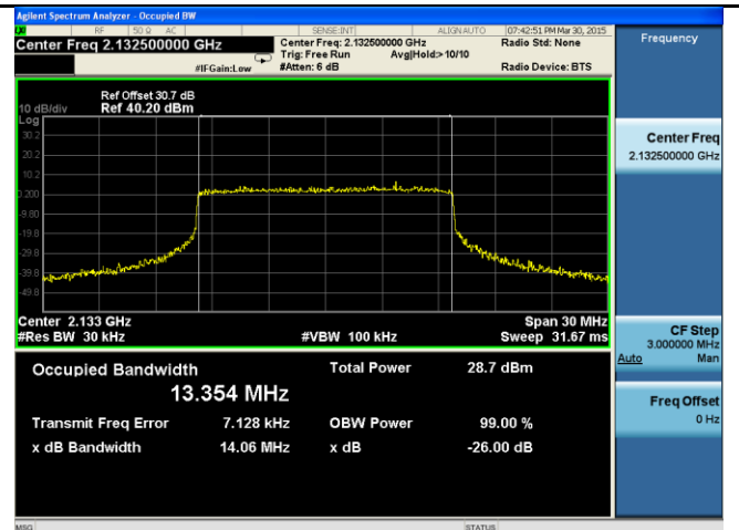
OBW-Band4-15M BW-Mid
