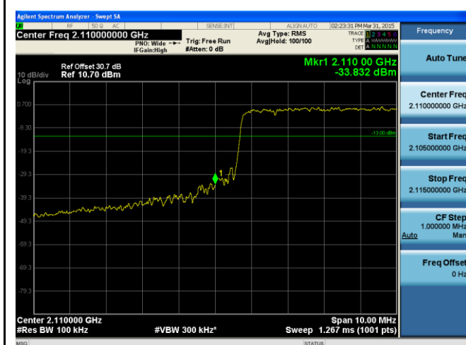
BandEdge-LTE-Band4-15MHz-64QAM-Low
