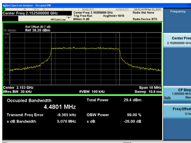
OBW-Band4-5M BW-High
