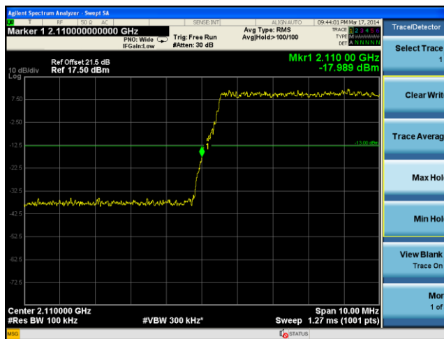
BandEdge-LTE-Band4-10MHz-64QAM-Low
