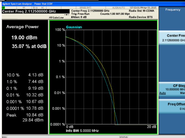
PK-AV-Ratio-Band4-64QAM-5M BW-Low
