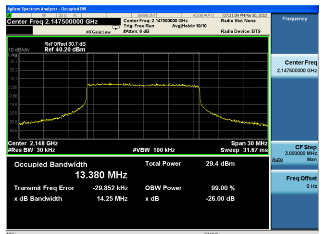
OBW-Band4-15M BW-High
