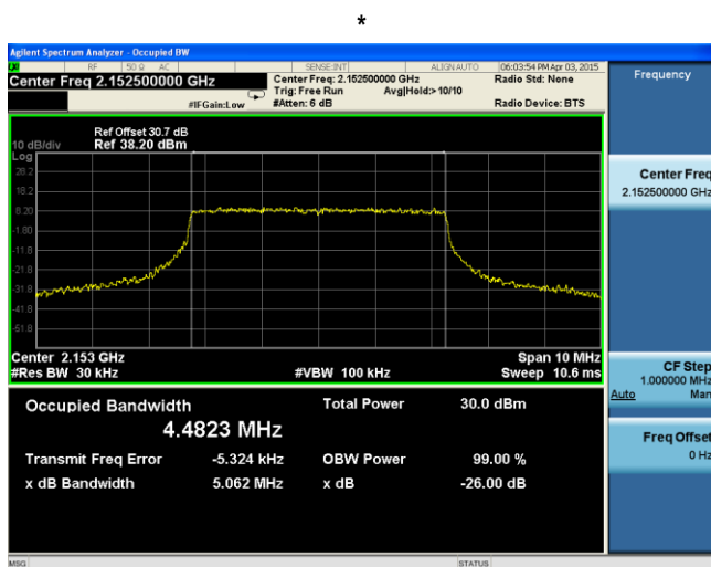
OBW-Band4-5M BW-High
