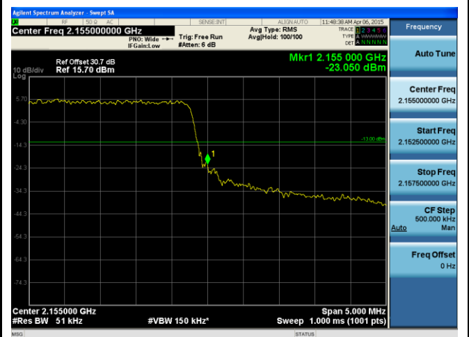
BandEdge-LTE-Band4-5MHz-64QAM-High
