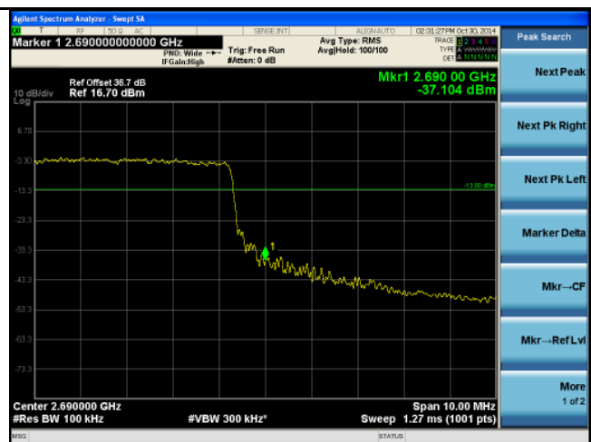
BandEdge-LTE-Band7-15MHz-64QAM-High – Chain B
