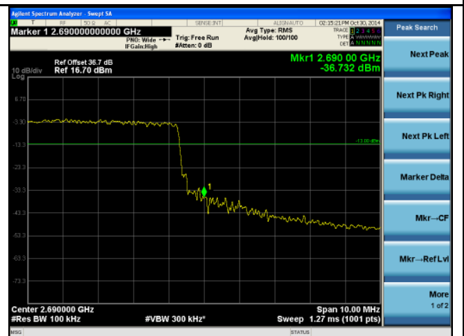
BandEdge-LTE-Band7-15MHz-QPSK-High – Chain B
