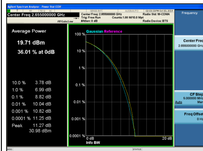
PK-AV-Ratio-Band7-64QAM-15M BW-Mid
