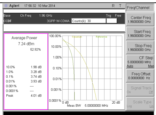
PK-AV-Ratio-Band2&25-QPSK-10M BW-Mid
