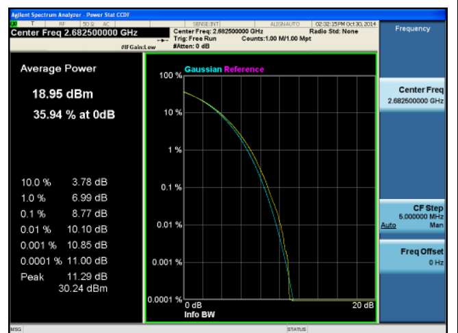
PK-AV-Ratio-Band7-64QAM-15M BW-High
