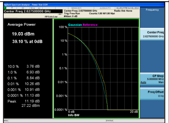
PK-AV-Ratio-Band7-64QAM-15M BW-Low
