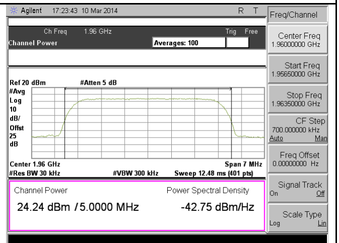
PWR-Band2&25-QPSK-Mid CH-Port2
