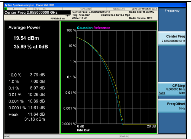
PK-AV-Ratio-Band7-QPSK-15M BW-Mid
