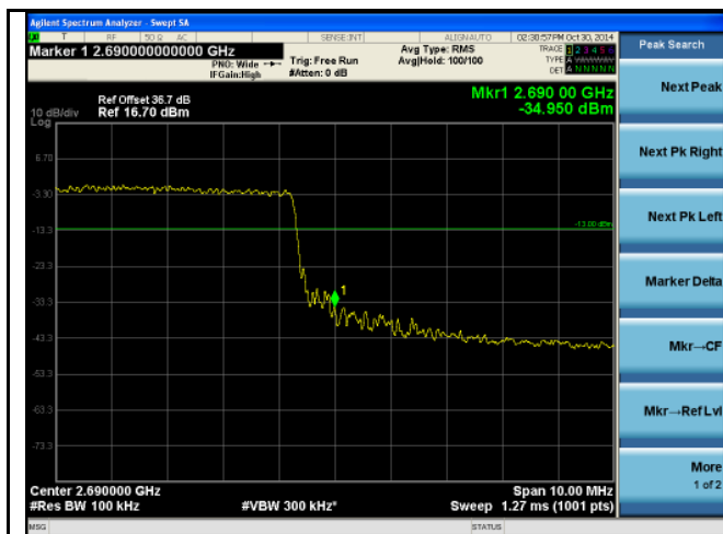
BandEdge-LTE-Band7-15MHz-64QAM-High – Chain A
