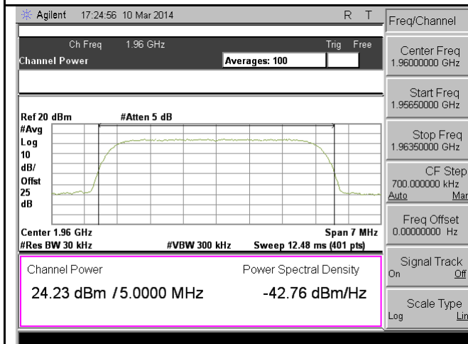
PWR-Band2&25-QPSK-Mid CH-Port1
