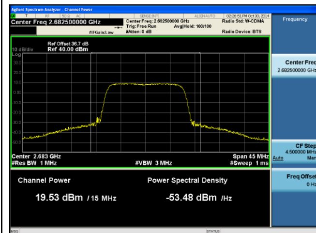
PWR-Band7-64QAM-15M BW-High CH-Port1
